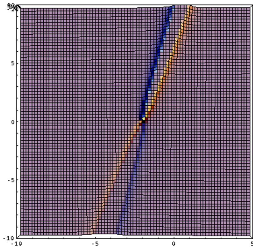
Figure 2: \frac{w_1(x,t)}{\sigma} with N = 1 , p_1 = 1 , s_1 = 2 and c = 0 .
