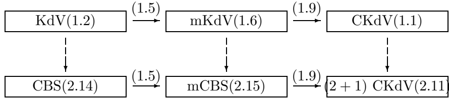
Figure 1: The dimensional extensions are indicated by broken arrows. These broken arrows indicate the modification of T operators for the search of the (2+1) -dimensional case. Full arrows mean the Miura transformations. The mKdV equation (6) and the mCBS equation (25) are induced by the Miura transformation (5) from the KdV equation (2) and CBS equation (24). We construct exact solutions of the CKdV equation (1) and the (2+1) -dimensional CKdV equation (21) from the solution of the mKdV equation (6) and the mCBS equation (25), by using using the Miura type transformation (9).
