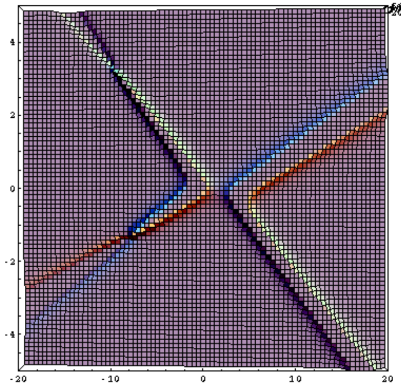
Figure 5: \frac{w_2(x, z, t)}{\sigma} with N = 2 , p_1 = 1 , q_1 = 3 , s_1 = 0 , p_2 = 0.5 , q_2 = -3 , s_2 = 0 , c = 0 and t = 0 .
