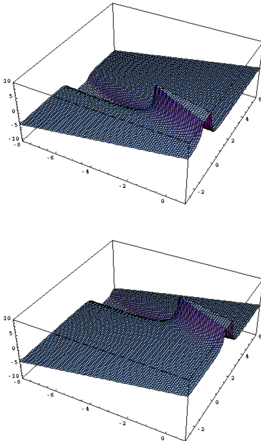
Figure 4: Time evolution of \frac{w_1(x, z, t)}{\sigma} with N = 1 , p_1 = 1 , q_1 = 3 , s_1 = 2 and c = 0 .
