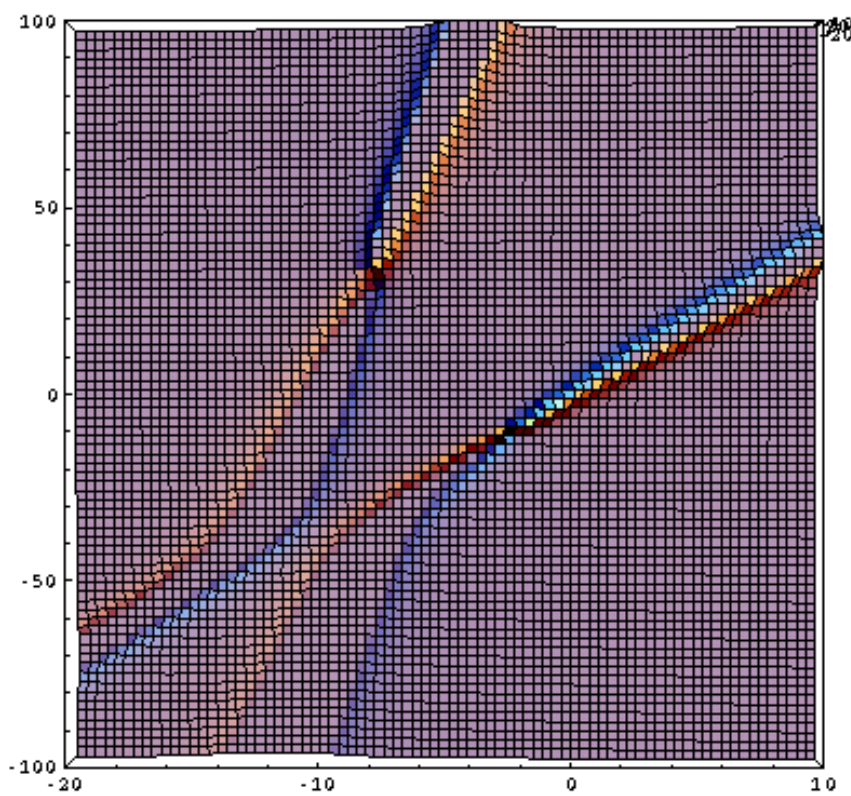
Figure 3: \frac{w_2(x, t)}{\sigma} with N = 2 , p_1 = 1 , s_1 = 2 , p_2 = 0.5 , s_2 = 5 and c = 0 .
