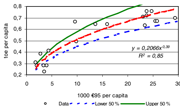
Fig 9. Dependence function of relative consumption of petroleum products in road transport (Ppt) on GDP per capita
