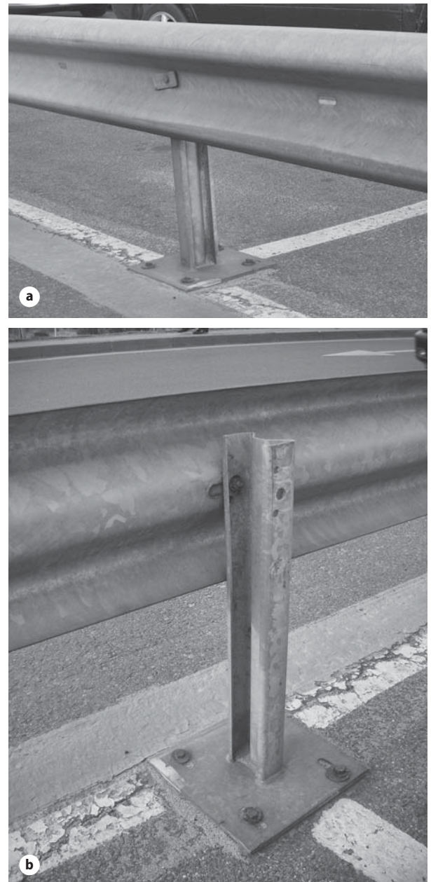
Fig. 5. The elements of metal guardrail: a – protective W-shape horizontal beam (in the foreground); b – \Sigma -shape post (in the foreground)
