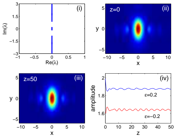
FIG. 4: Demonstration of stability for the embedded soliton in Fig. 3(B). (i) the linear-stability spectrum, showing that this soliton is linearly stable; (ii) an initially perturbed embedded soliton (6) with \epsilon = 0.2 ; (iii) evolution of the perturbed soliton in (ii) at z = 50 ; plotted in (ii, iii) are |U| fields; (iv) peak-amplitude evolutions of the perturbed embedded soliton (6) for \epsilon = 0.2 and -0.2 .
