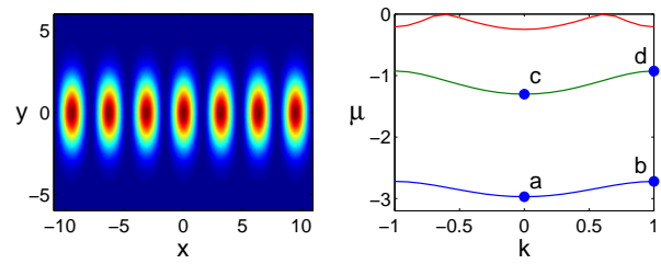
FIG. 1: Left: the quasi-1D waveguide array n(x, y) in our model. Right: the Bloch bands in this waveguide. The edges of the lowest two Bloch bands are marked by letters 'a-d'.
