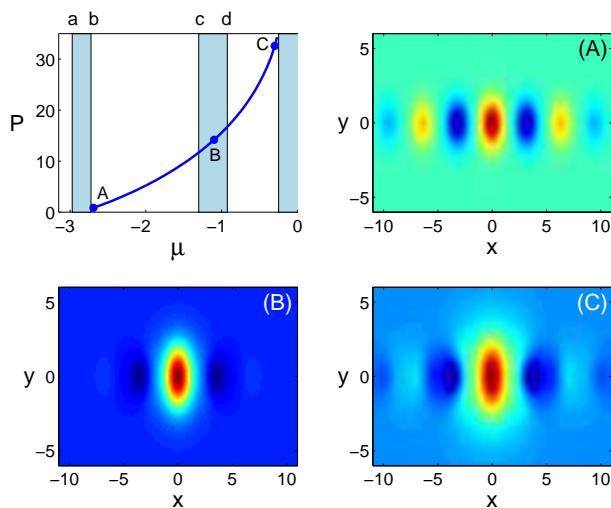
FIG. 3: A soliton family under self-defocusing nonlinearity ( \sigma = -1 ). Upper left panel: the power curve; the shaded stripes indicate Bloch bands, and the band edges marked by ‘a-d’ on top of the panel correspond to the edges of the same marker in Fig. 1. Panels (A-C) are soliton profiles u(x, y) at locations marked by the same letters on the power curve. The soliton at location ‘B’ is an embedded soliton which is fully localized in both x and y dimensions.
