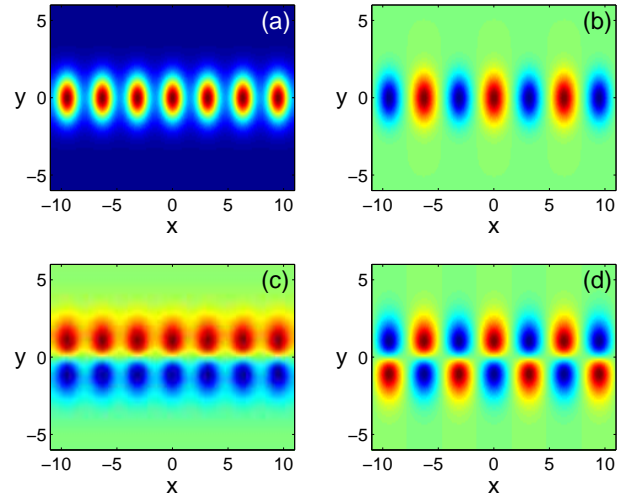
FIG. 2: Bloch modes at edges 'a-d' of the lowest two Bloch bands in Fig. 1 respectively.
