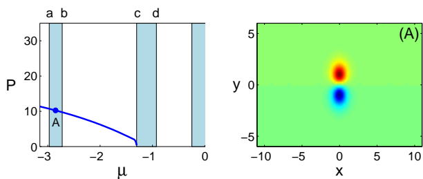
FIG. 5: 2D embedded solitons under self-focusing nonlinearity ( \sigma = 1 ). Left panel: the power curve of this soliton family (same notations as Fig. 3); right panel: an embedded soliton in the first Bloch band (at location ‘A’ of the power curve).
