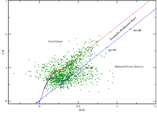
Fig. 4. (H-K, J-H) color-color diagram of the 2MASS sources found in a 400'' circular area centered at (l, b) = (91^\circ.7, 1^\circ.83) . The two solid curves represent the location of the main sequence (blue line) and the giant stars (red line) derived from ?. The parallel dashed lines are reddening vectors with the crosses placed at intervals corresponding to five magnitudes of visual extinction. We assumed the interstellar reddening law of ?, A_J/A_V = 0.282 and A_H/A_V = 0.175 .
