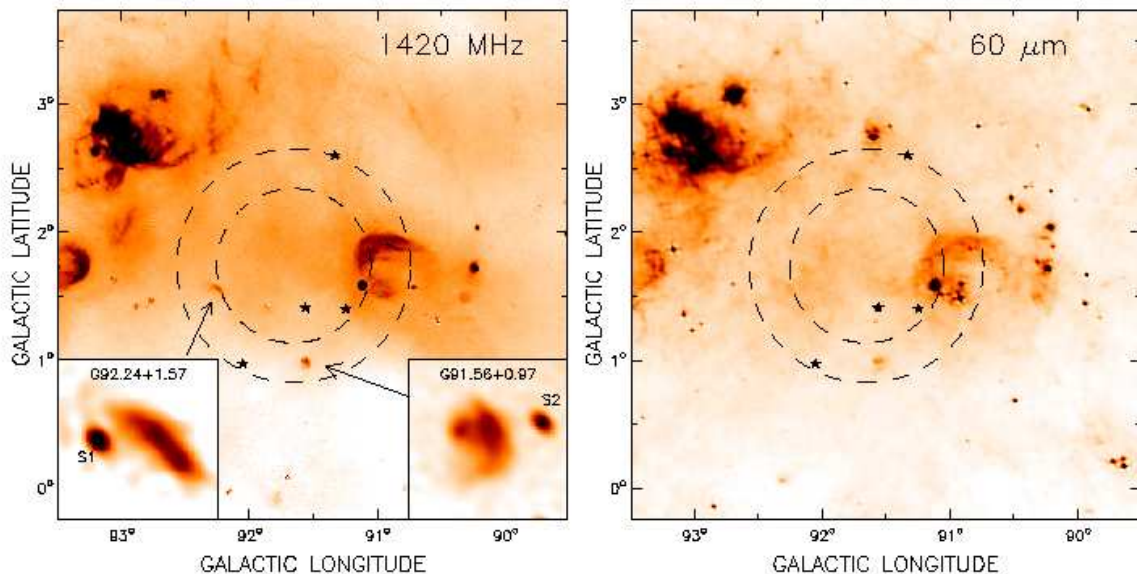
Fig. 3. 1420 MHz radio continuum and 60 \mu\text{m} images from the CGPS survey. Resolution for both is about 1' . Point-like sources have been removed from the radio continuum image. Circles indicate the approximate inner and outer boundary of the HI shell seen in Figure 1. The two insets at the bottom of the radio image show a close-up view of G91.56+0.97 and G92.24+1.57 (point-like sources included, see text).
