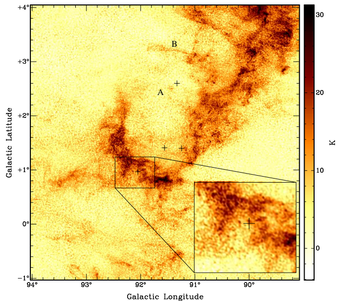
Fig. 1. HI emission distribution averaged between -110.3 and -116.9 \text{km s}^{-1} . The plus symbols indicate the position of the four DWCL source candidates, IRAS 21147+5016, IRAS 21106+5013, IRAS 21093+4959, and IRAS 21041+5052. The inset is a close-up view of the region near IRAS 21147+5016.
