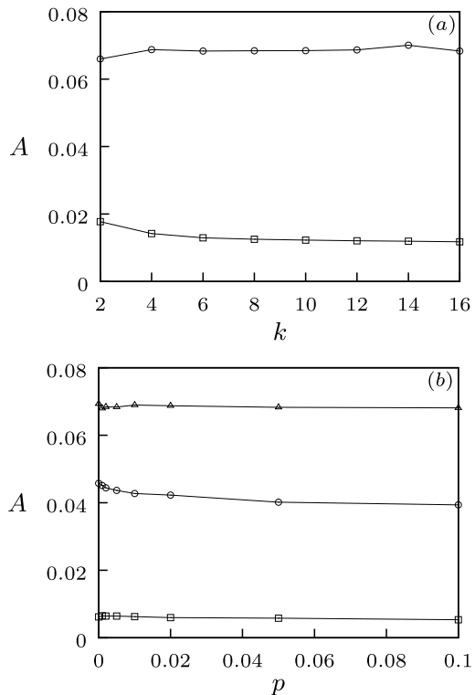
FIG. 3: (a) Activity as a function of k , on a regular lattice with p = 0 , fixed f = 0.5 , and for different values u = 1 (squares) and u = 10 (circles). (b) Activity as a function of p , on a network with k = 4 , and for different values f = 0.5 (triangles), f = 0.3 (circles) and f = 0.1 (squares).
