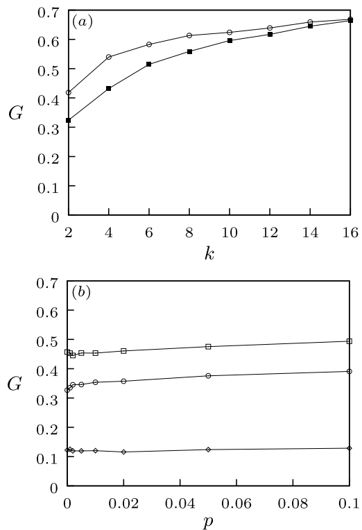
FIG. 5: (a) Gini coefficient at t = 10^8 as a function of k on a regular lattice with p = 0 , for f = 0.1 , u = 1 (squares) and u = 10 (circles). (b) Gini coefficient at t = 10^8 as a function of the rewiring probability p on a network with k = 4 , with fixed u = 10 and f = 0.5 (diamonds), f = 0.3 (circles), and f = 0.1 (squares).
