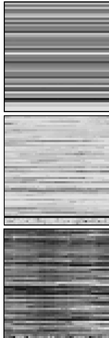
FIG. 1: Spatiotemporal patterns in a one-dimensional lattice with k = 2 , size N = 50 and W = 1 , after discarding 5000 time steps. The vertical axis describes the ordered position i of the agents in the lattice, increasing from bottom to top. Horizontal axis represents time, increasing from left to right. The wealths w_i(t) evolving in time are represented by a color code. The color palette goes from light gray (the poorest agent) to dark gray (the richest agent). Top: laminar state; u = 10 , f = 0.001 . Center: spatiotemporal intermittent state; u = 3 , f = 0.4 . Bottom: turbulent state; u = 30 , f = 0.4 .
