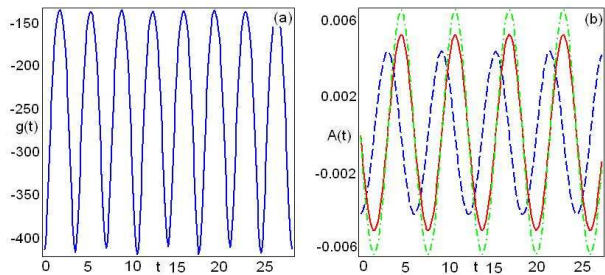
FIG. 3: (color online). Profiles of (a) nonlinearity g(t) given by Eq. (7b) and (b) the coefficients A_x(t) (solid line), A_y(t) (dashed line), and A_z(t) (dashed-dotted line) of second degree term of the linear potential v(\mathbf{r}, t) given by Eq. (8) vs time for the parameters are given by Eq. (14).
