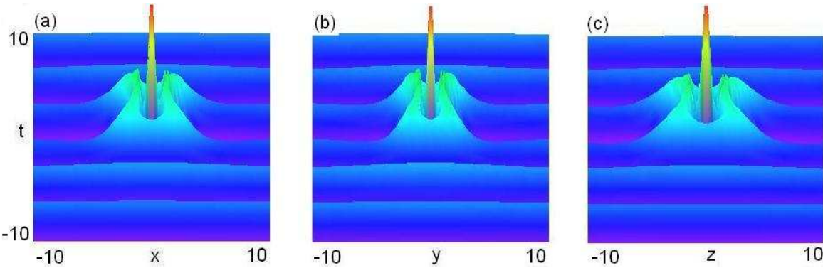
FIG. 6: (color online). Color coded wave intensity (a) |\Psi_2|^2(x, 0, 0, t) with \max_{\{x,0,0,t\}} |\Psi_2|^2 = 0.038 , (b) |\Psi_2|^2(0, y, 0, t) with \max_{\{0,y,0,t\}} |\Psi_2|^2 = 0.036 and (c) |\Psi_2|^2(0, 0, z, t) with \max_{\{0,0,z,t\}} |\Psi_2|^2 = 0.038 given by the solution (15) for a_\sigma(t) = 0 and other parameters given by Eq. (14).
