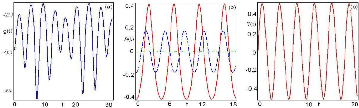
FIG. 1: (color online). Profiles of (a) nonlinearity g(t) given by Eq. (7b), (b) the coefficients A_x(t) (solid line), A_y(t) (dashed line), and A_z(t) (dashed-dotted line) of second degree term of the linear potential v(\mathbf{r}, t) given by Eq. (8) and (c) the gain/loss term \gamma(t) vs time for the parameters are given by Eq. (13) with k_x = 0.9 , k_y = 0.6 , k_z = 0.1 and k = 0.6 .
