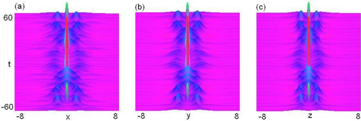
FIG. 5: (color online). Color coded wave intensity (a) |\Psi_2|^2(x, 0, 0, t) with \max_{\{x,0,0,t\}} |\Psi_2|^2 = 0.135 , (b) |\Psi_2|^2(0, y, 0, t) with \max_{\{0,y,0,t\}} |\Psi_2|^2 = 0.13 and (c) |\Psi_2|^2(0, 0, z, t) with \max_{\{0,0,z,t\}} |\Psi_2|^2 = 0.125 given by the solution (15) for a_\sigma(t) = 0 and other parameters given by Eq. (13) with k_x = 0.9 , k_y = 0.6 , k_z = 0.1 and k = 0.6 .
