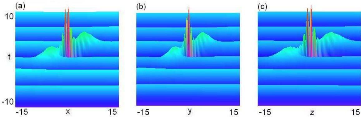
FIG. 4: (color online). Color coded plot of wave intensity (a) |\Psi_1|^2(x, 0, 0, t) with \max_{\{x,0,0,t\}} |\Psi_1|^2 = 0.027 , (b) |\Psi_1|^2(0, y, 0, t) with \max_{\{0,y,0,t\}} |\Psi_1|^2 = 0.03 and (c) |\Psi_1|^2(0, 0, z, t) with \max_{\{0,0,z,t\}} |\Psi_1|^2 = 0.029 defined by the solution (12) for the parameters given by Eq. (14).
