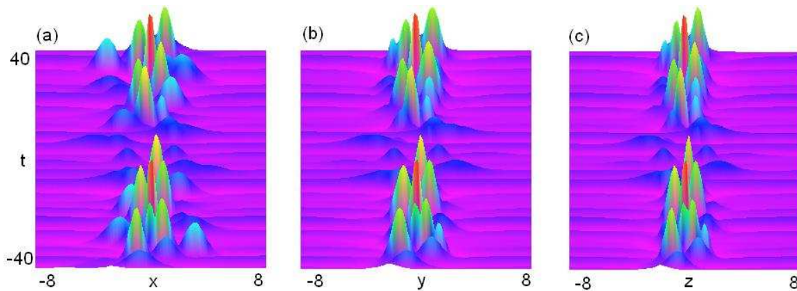
FIG. 2: (color online). Color coded plot of wave intensity (a) |\Psi_1|^2(x, 0, 0, t) with \max_{\{x,0,0,t\}} |\Psi_1|^2 = 0.06 , (b) |\Psi_1|^2(0, y, 0, t) with \max_{\{0,y,0,t\}} |\Psi_1|^2 = 0.068 and (c) |\Psi_1|^2(0, 0, z, t) with \max_{\{0,0,z,t\}} |\Psi_1|^2 = 0.068 defined by the solution (12) for the parameters given by Eq. (13) with k_x = 0.9 , k_y = 0.6 , k_z = 0.1 , k = 0.6 . Note that for given set of parameters, the wave is localized in space.
