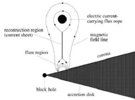
Fig. 1. The CME bubble is connected to the low-lying loops via an extended current sheet (Yuan et al. 2009).
