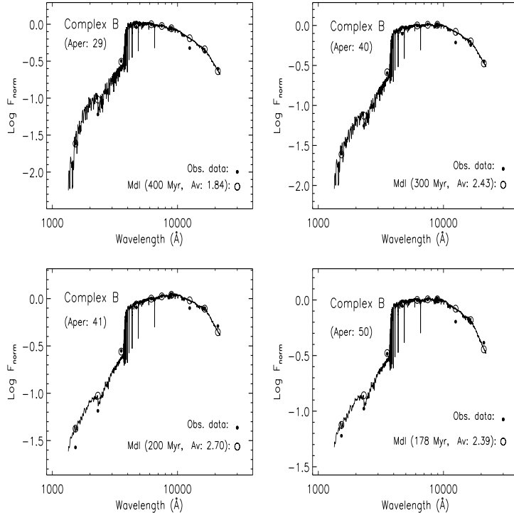
Fig. 7.— Similar to Fig. 6, but for some apertures located inside complex B.
