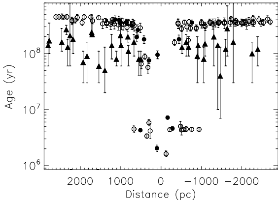
Fig. 9.— Derived ages of the dominant stellar population within apertures of 5'' radius as a function of the distance to the galactic center (positive distances correspond to the north-east direction). Circles mark the results for the selected apertures, with the filled circles marking the complexes defined by O’Connell & Manganó (1978). Ages of the clusters from Konstantopoulos et al. (2009) are denoted by triangles.
