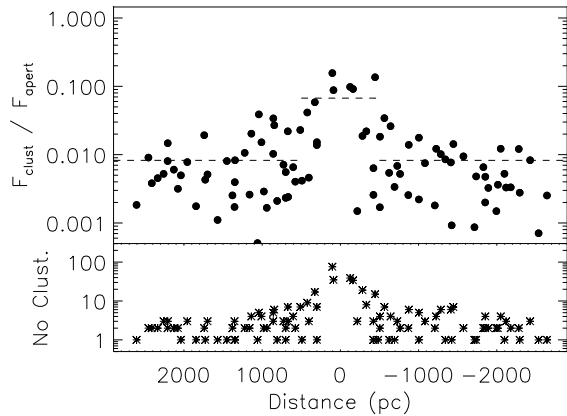
Fig. 14.— The contribution to the total flux by the stellar clusters as a function of the distance to the galactic center (each point corresponds to an aperture). The upper plot shows that the mean contribution in the nucleus is \sim 7\% , whereas in the disk it is around 0.7\% (dashed lines). The lower plot shows the number of star clusters inside each aperture (as in previous figures, positive distances correspond with the NE).
