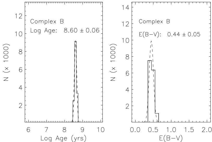
Fig. 3.— Age and color excess obtained for complex B (aperture 27). The Monte-Carlo simulation provides several best-fit models. The fitted gaussian (dashed line) gives us the value of the age (left) and extinction (right) and their corresponding errors.
