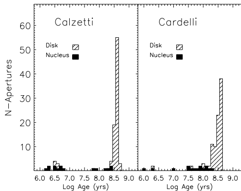
Fig. 5.— Ages of the apertures obtained using Calzetti (left) and Cardelli (right) attenuation curves. Both the curves give similar ages for disk, whereas Cardelli curve gives systematically higher ages ( \sim 10^8 yr instead of \sim 10^6 yr) for nuclear apertures.
