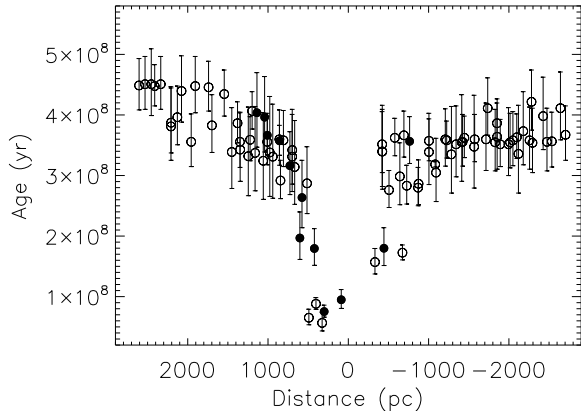
Fig. 10.— As in previous Figure, but with the vertical axis on a linear scale to enable better visualization of a slightly outside-in age gradient in the disk of M82.
