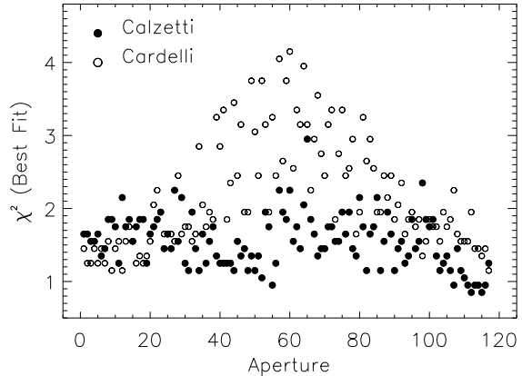
Fig. 4.— The minimum \chi^2 values obtained using Calzetti (solid circles) and Cardelli (open circles) extinction curves for all the selected apertures. Calzetti attenuation curve provides lower \chi^2 values, especially in the dusty central zone (apertures 30-90).
