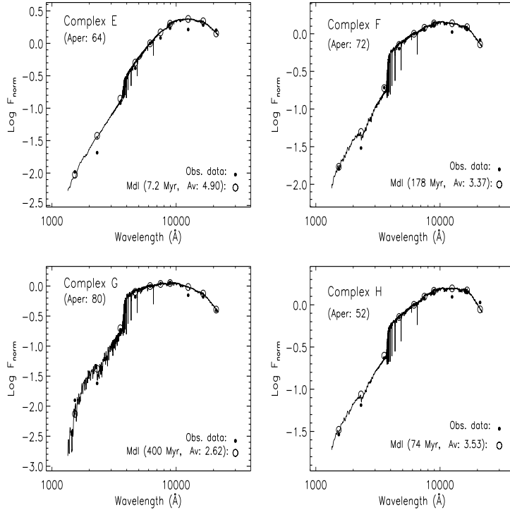
Fig. 8.— Similar to Fig. 6, but for complexes E, F, G and H.
