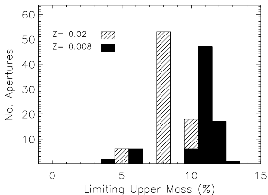
Fig. 13.— The histogram shows the limiting upper masses of old population that can be added to the best-fit SSP of apertures located in the disk of M82. The mean value is 9% for solar metallicity models and 11% for metal-poor models.
