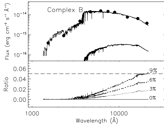
Fig. 12.— The observed SED (circles) of an area of complex B (aperture 27) is plotted in the upper panel, as well as the SED of the best-fit SSP (solid line fitting the dots) and the SED of the old population model (solid line) with 9% in mass of the best-fit model. The lower panel shows the ratio ( F_{Old-Pop}/F_{Best-Fit} ) for different fractional masses (indicated as percentage for each curve) of the old population. For the aperture plotted, a mass > 9\% would have been noticed in the K-band photometry.
