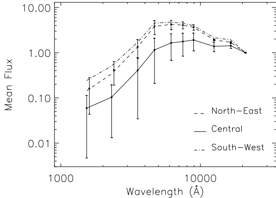
Fig. 2.— Mean SEDs across the M82 disk. Solid line represents the mean of SEDs for selected nuclear apertures. Dashed and dot-dashed lines are the mean SEDs for apertures located in the north-east and south-west of M82 respectively. The mean SEDs were normalized in the K-band flux and the vertical bars represent the flux dispersion ( 1\sigma ).
