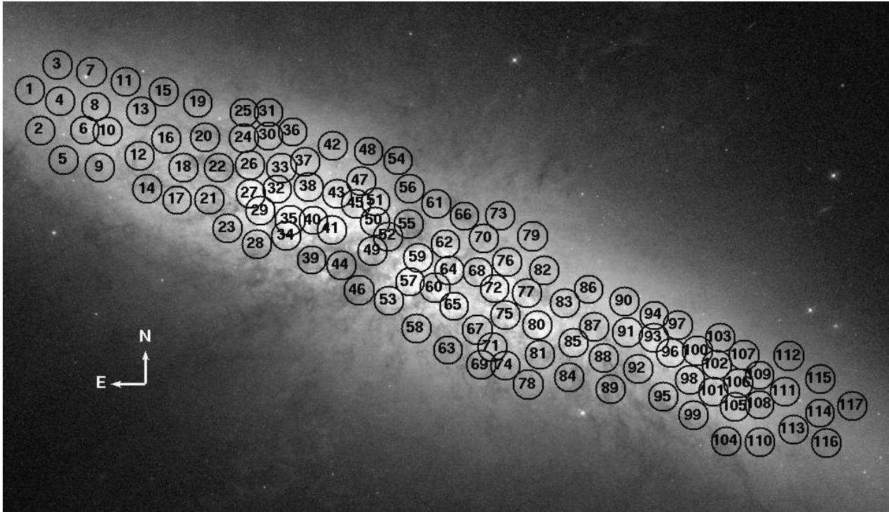
Fig. 1.— F555W image of M82 from HST . The positions of the 117 apertures ( 5'' radius) defined in this work are marked with circles. The classical M82 complexes A, C, D, E, F, G, and H correspond to the apertures 57, 65, 59, 64, 72, 80 and 52 respectively. The complex B contains the apertures 27, 29, 32, 35, 40, 41, 45 and 50.
