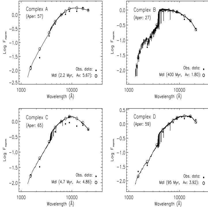
Fig. 6.— The observed SEDs for complexes A, B, C and D (solid circles) are compared with the best-fit model SED (open circles) and the corresponding full resolution model spectrum (solid line). The derived age and extinction are given in each plot.
