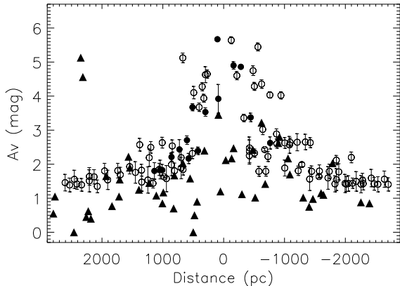
Fig. 11.— The visual extinction within apertures of 5'' radius as a function of the distance to the galactic center (positive distances correspond to the north-east direction). The central part of the galaxy is more extinguished, A_V > 3.5 mag. Circles describe our results, filled circles are related to named complexes, and triangles represent A_V in clusters obtained by Konstantopoulos et al. (2009).
