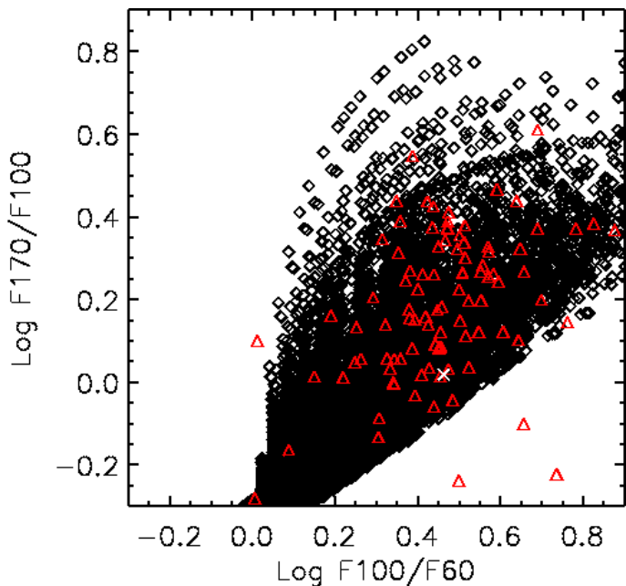
Fig. 20. The 170/100 versus 100/60 micron colour-colour plot for our simulated SEDs (black diamonds). Overplotted with red triangles are the observed colours of the spiral galaxies from the ISOPHOT Virgo Cluster Deep Survey (IVCDS; Tuffs et al. 2002a, 2002b; Popescu et al. 2002) and the ISOPHOT Serendipity Survey (Stickel et al. 2000). Only spiral galaxies with Hubble type earlier than Sd are plotted. The white star represents the position of NGC 891 in the colour-colour diagram.
