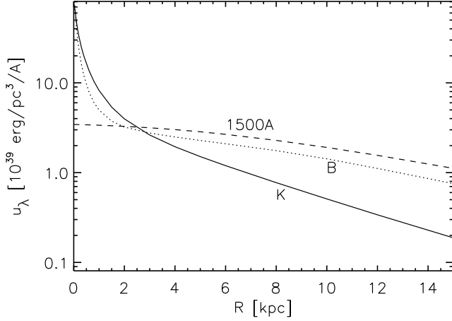
Fig. 4. Examples of calculated radial profiles of radiation fields in the plane of the disk ( z = 0 pc), for the best fit model of our prototype galaxy NGC 891. The different profiles are for different wavelengths.
