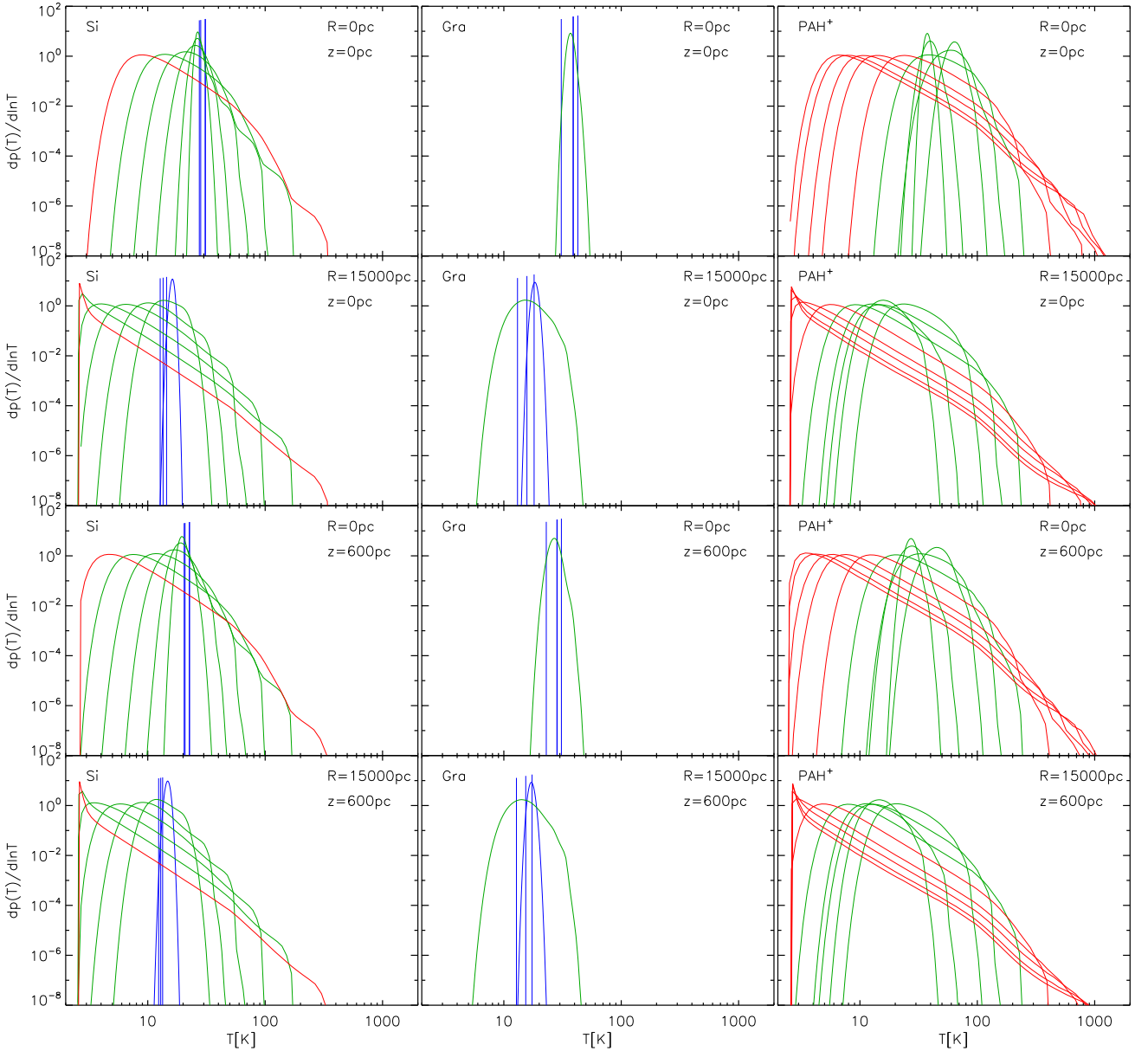
Fig. 6. Temperature distributions for dust grains of different sizes (plotted as different curves in each panel) and various composition: Si (left panels), Gra (middle panels) and PAH + (right panels), heated by the diffuse radiation fields calculated for the best fit model of our prototype galaxy NGC 891. Temperature distributions for PAH 0 are not plotted in this figure. The colour coding is as follows: red is for grains with radius a < 0.001 \mu\text{m} (0.00035, 0.00040, 0.00050, 0.00063 and 0.00100 \mu\text{m} ), green is for grains with 0.001 < a \leq 0.01 (0.00158, 0.00251, 0.00398, 0.00631, 0.01000 \mu\text{m} ) and blue is for grains with a > 0.01 (0.0316, 0.10000, 0.31623, 0.7943 \mu\text{m} ). The biggest grains have delta function distributions, since they emit at equilibrium temperature. Going from the top to the bottom panels the calculations are done for different positions in the model galaxy: R = 0 \text{ pc} , z = 0 \text{ pc} ; R = 15000 \text{ pc} , z = 0 \text{ pc} ; R = 0 \text{ pc} , z = 600 \text{ pc} ; and R = 15000 \text{ pc} , z = 600 \text{ pc} .
