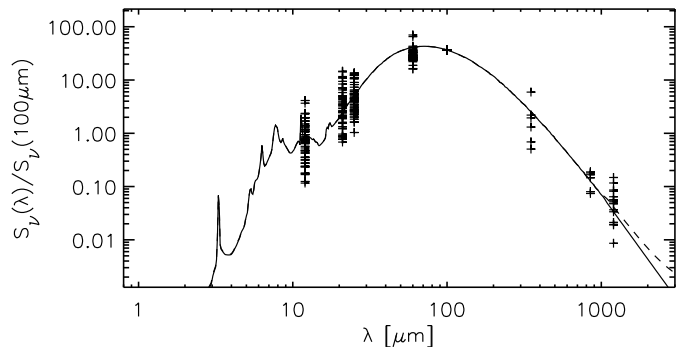
Fig. 3. MSX and IRAS mid-IR and far-IR integrated photometry for 57 SF regions from Conti & Crowther (2004), supplemented by all published sub-mm and/or near-mm data for which integrated flux measurements covering the full angular extent of the source are available (18 sources); (see Table 1). Measurements are normalised to the 100\mu\text{m} flux density. The solid line is the adopted model for the PDR dust, PAH emission from Groves et al. (2008), having compactness parameter \log(C) = 6.5 , metallicity 1.0, and PDR column density \log(N) = 22.0 . The dashed-line, which deviates slightly from the solid line in the submm range, is the same but with the free-free emission included.
