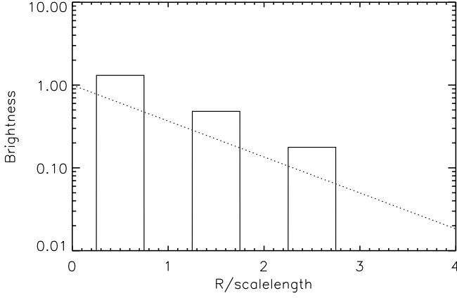
Fig. 11. The radial distribution used to test the effect of a spiral pattern for the young stars and associated diffuse dust (solid line), overplotted on the distribution for the standard model with an exponential disk (dotted line). The radial coordinate is given in units of exponential scalelengths, where the scalelength of the exponential disk is h^{\text{disk}} = 5670 pc.
