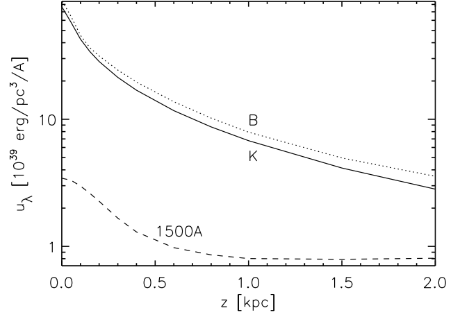
Fig. 5. Examples of calculated vertical profiles of radiation fields in the centre of the disk ( R = 0 pc), for the best fit model of our prototype galaxy NGC 891. The different profiles are for different wavelengths.
