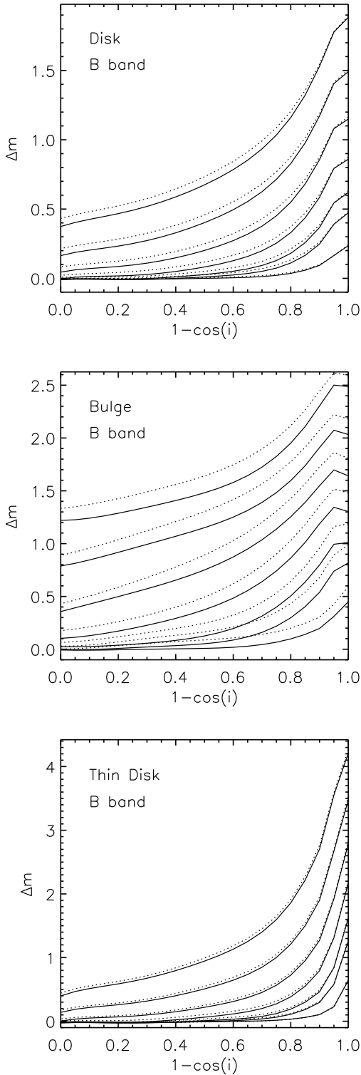
Fig. B.1. The attenuation-inclination relation for the disk (top), bulge (middle) and thin disk (bottom) in the B band. In each panel the solid curves represent the attenuations calculated with the dust model used in this paper, incorporating a mixture of silicate, graphite and PAH molecules. The dotted curves represent the corresponding attenuations calculated with the dust model used in Paper III, incorporating only a mixture of silicates and graphites. In each panel the 7 different curves represent the attenuation-inclination relations for different \tau_B^f : 0.1, 0.3, 0.5, 1.0, 2.0, 4.0, 8.0, with the values increasing from bottom curves to top curves.
