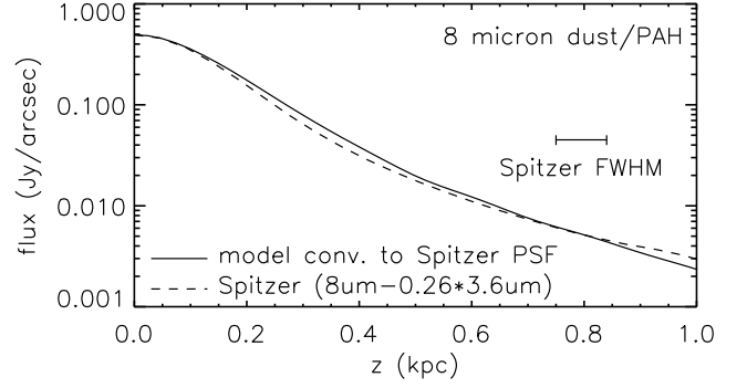
Fig. 9. Comparison between the 8 \mu\text{m} Spitzer vertical profile of NGC 891 integrated over longitude (dashed line) and our corresponding model predictions (solid line). Before comparison with the model, the 8 \mu\text{m} image had the stellar component subtracted off.
