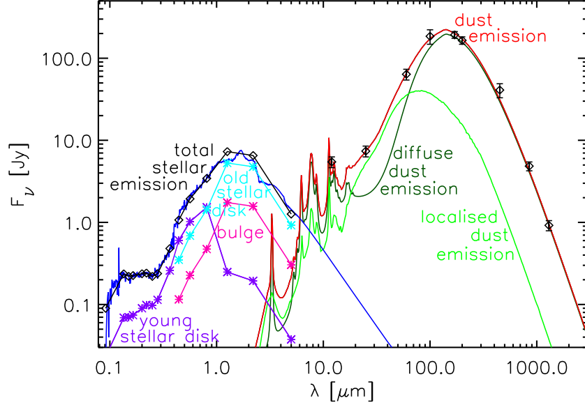
Fig. 8. The best fit model SED of NGC891, corresponding to \tau_B^f = 3.5 , SFR = 2.88 M_\odot/\text{yr} , F = 0.41 , together with the observed data in the MIR/FIR/submm (plotted as rhombus symbols with error bars). The observed flux densities and the corresponding references are given in Table 1. The calculated total intrinsic stellar SED is plotted as black line and rhombus symbols. The predicted stellar SED given by population synthesis models is plotted as dark blue line. The intrinsic stellar SED of the young stellar population in the diffuse component (the fraction 1 - F escaping the star-forming complexes) is plotted with mauve line. The intrinsic SED (only diffuse) of the old stellar population, as derived from the optimisation of the optical/NIR images of NGC891, is plotted with light blue line. The corresponding SED for the bulge is plotted with pink line. The different symbols overlapped on the UV/optical SEDs indicate the wavelength at which the radiative transfer calculations were performed. The predicted PAH and dust emission SED is given with red line. Also plotted are the two main components of infrared emission: the predicted diffuse SED (dark-green line) and the predicted clumpy component associated with the star-forming regions (light-green line).
