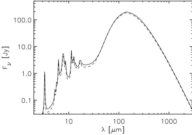
Fig. 12. Comparison between model solutions for the dust emission SEDs calculated under the assumption that the emissivity of the young stellar population and the opacity of the associated dust are distributed in a thin disk (solid line) and in a spiral pattern (dashed line), respectively. The solution is for the best fit of NGC 891.
