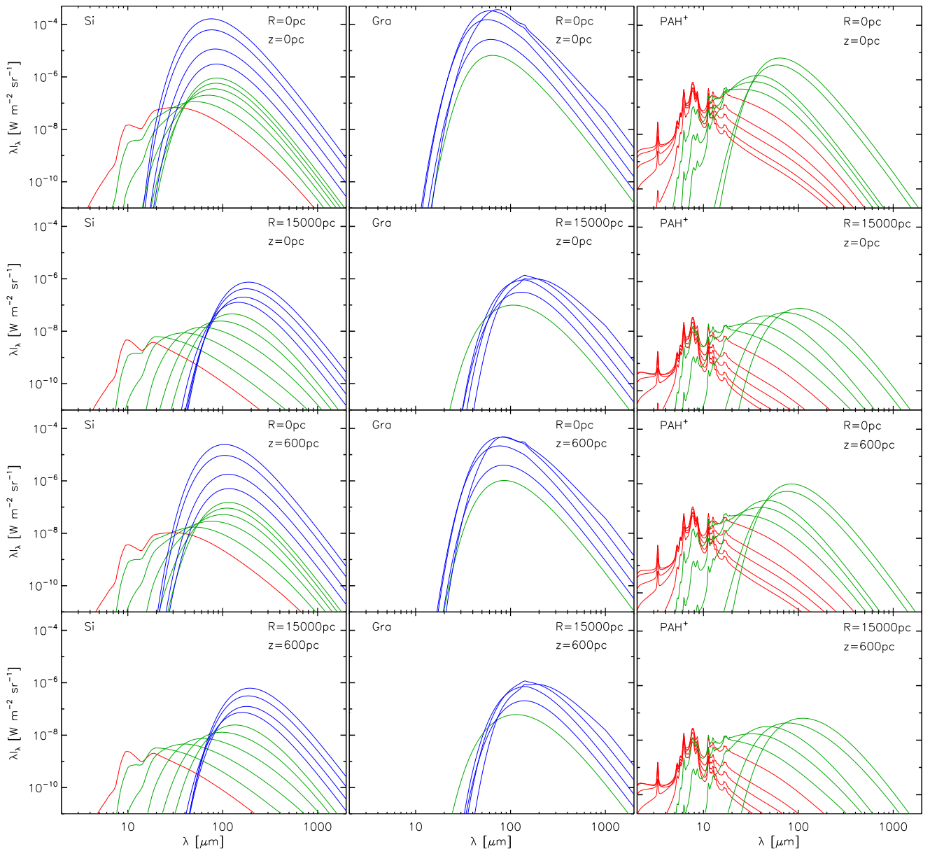
Fig. 7. Infrared brightnesses for grains of different sizes (plotted as different curves in each panel) and various composition: Si (left panels), Gra (middle panels) and PAH + (right panels), heated by the diffuse radiation fields calculated for the best fit model of our prototype galaxy NGC 891. Infrared brightnesses for PAH 0 are not plotted in this figure. The colour coding is as follows: red is for grains with radius a < 0.001 \mu\text{m} (0.00035, 0.00040, 0.00050, 0.00063 and 0.00100 \mu\text{m} ), green is for grains with 0.001 < a \leq 0.01 (0.00158, 0.00251, 0.00398, 0.00631, 0.01000 \mu\text{m} ) and blue is for grains with a > 0.01 (0.0316, 0.10000, 0.31623, 0.7943 \mu\text{m} ). The grain sizes considered in this plot are the same as those plotted in Fig. 6. Going from the top to the bottom panels the calculations are done for different positions in the model galaxy: R = 0 \text{ pc} , z = 0 \text{ pc} ; R = 15000 \text{ pc} , z = 0 \text{ pc} ; R = 0 \text{ pc} , z = 600 \text{ pc} ; and R = 15000 \text{ pc} , z = 600 \text{ pc} .
