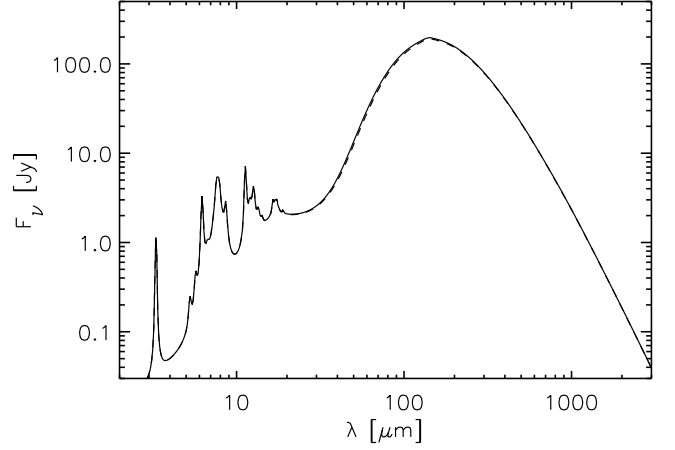
Fig. 13. Comparison between model solutions for dust emission SEDs calculated using intrinsic SEDs of the old stellar population peaking in the J (solid line) and K band (dashed line), respectively. The solution is for the best fit of NGC 891.
