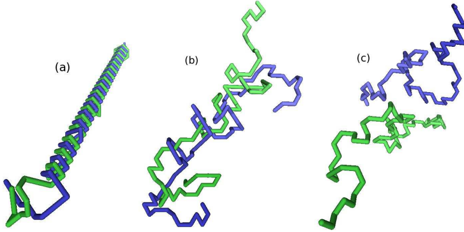
FIG. 1: (Color online) Snapshots of the polymer configurations during unwinding for two strands of length N = 100 each. The initial conformation is fully double helical all along its length. (a) Snapshot after short time from the beginning of the simulation; opening begins mainly from the two ends, although small bubbles within the chain are also visible. (b) Snapshot at later times. (c) Separation.
