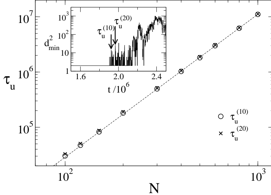
FIG. 2: Double-logarithmic plot of the average unwinding time as a function of strand length. The circles are obtained with an unwinding threshold of d_0^2 = 10 , while the crosses correspond to a threshold of d_0^2 = 20 . The straight dashed line is a fit to the data corresponding to an unwinding exponent of \beta = 2.57 . Inset: Plot of d_{\min}^2(t) vs. time for a run with strands of length N = 500 . The arrows indicate the first time that this distance reaches its threshold value d_0^2 = 10 or 20 .
