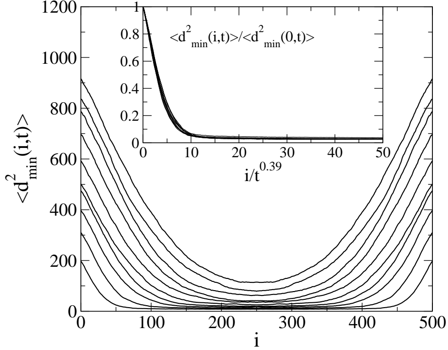
FIG. 4: Average squared minimal distance \langle d_{\min}^2(i, t) \rangle as a function of monomer number i , for polymers with length N = 500 . From bottom to top, the curves are obtained at times t/10^5 = 1, 2 \dots 10 . Inset: Collapse of \langle d_{\min}^2(i, t) \rangle / \langle d_{\min}^2(0, t) \rangle for polymers of length N = 1000 again at times t/10^5 = 1, 2 \dots 10 . The vertical scale is normalized so that all curves start from a common value at i = 0 . The horizontal scale is divided by t^{0.39} . This exponent is consistent with that obtained from the scaling of the unwinding time.
