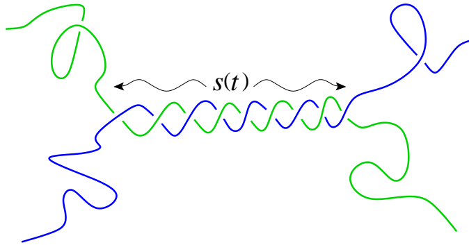
FIG. 3: Sketch of a double-stranded polymer during the unwinding dynamics. At time t we expect to find a double stranded region of curvilinear length s(t) terminates with two single strands of lengths (N - s(t))/2 at both edges, s(t) being a decreasing function of t .
