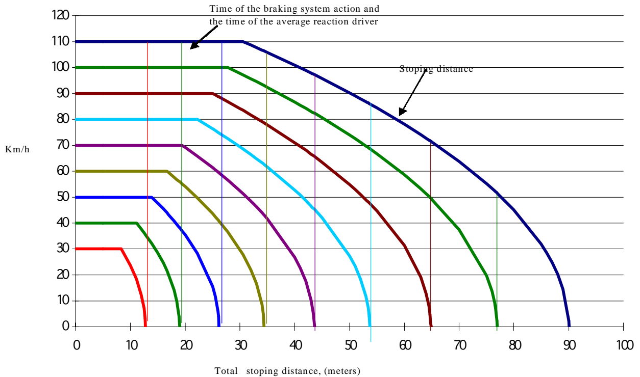
Fig 1. Average vehicle stopping distance (drivers reaction time and stopping distance)
