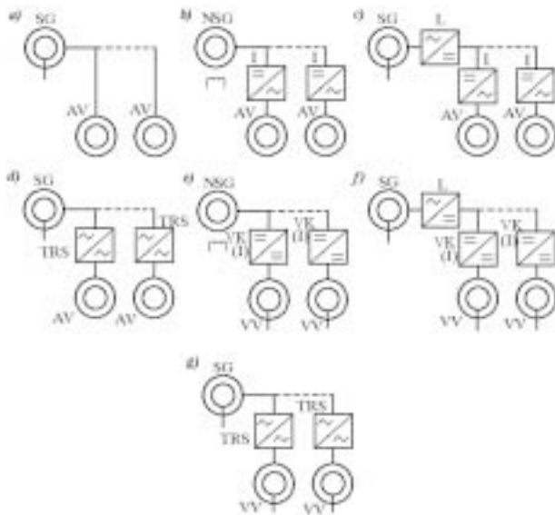
Fig 1. Types of diesel locomotive electric drives used with non-commutator traction motors:
