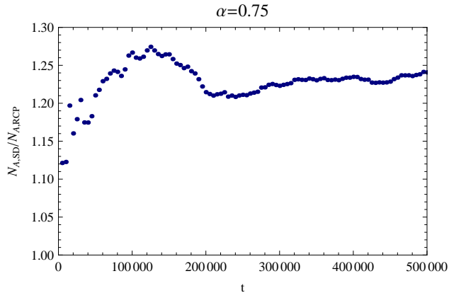
FIG. 4: Quotient of total amount of A-particles for the subdiffusive case and subdiffusion with randomized particles \frac{N_{A,SD}}{N_{A,RCP}} as a function of time.
