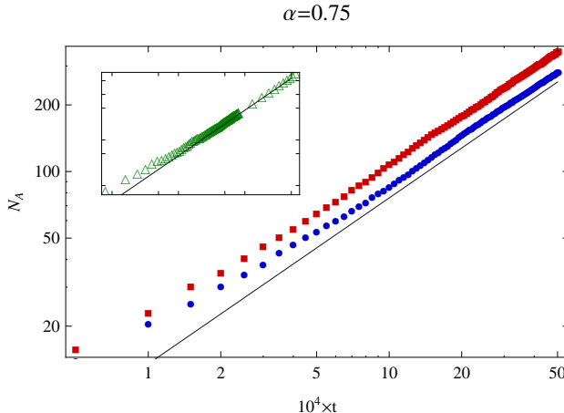
FIG. 2: Time dependence of the total amount of A-particles N_A for the subdiffusive case (squares) and subdiffusion with randomized particles (circles). The black line denotes the theoretical curve according to (31). The inset shows the situation for an exponential waiting time pdf (with mean 1), t goes from 10 to 5 \times 10^4 , N_A goes from 6 to 2000. The black line denotes again the theory, N_A = Dc^2t ; c = 0.3 .
