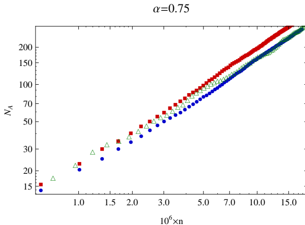
FIG. 3: Total amount of A-particles N_A for the normal case (triangles), the subdiffusive case (squares) and subdiffusion with randomized jumps (circles), both \alpha = 0.75 , depending on the total number of performed steps; c = 0.3 .
