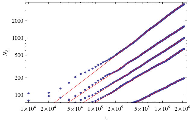
FIG. 1: Front position for \alpha = 0.9, 0.8, 0.75, 0.7, 0.6 (upper to lower graphs), c = 0.3 . Red lines denote fits of the large time behavior.
