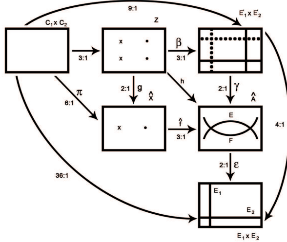
Figure 2: The product-quotient construction
