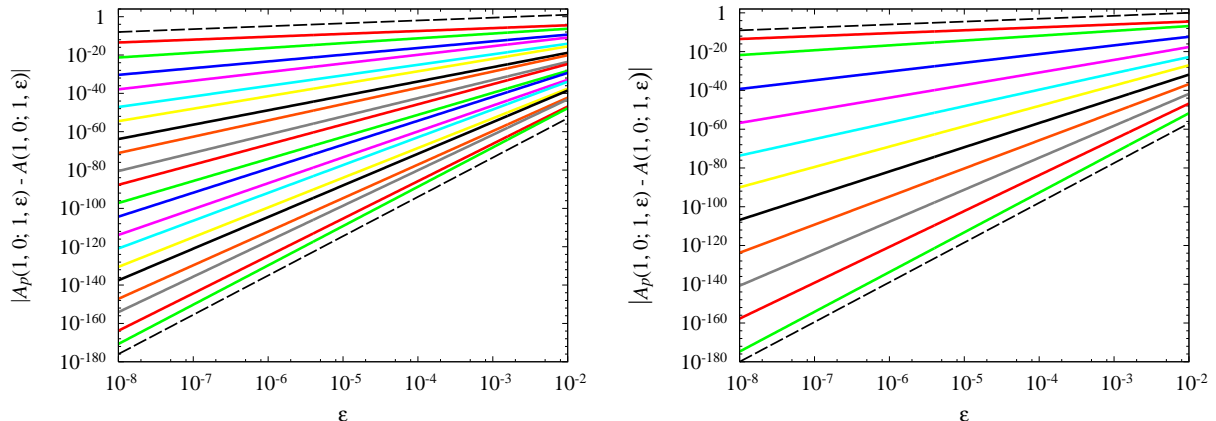
Figure 2: Deviations of diagonal transition amplitudes |A_p(1, 0; 1, \varepsilon) - A(1, 0; 1, \varepsilon)| as a function of propagation time \varepsilon : (left) time-dependent harmonic oscillator (56), calculated analytically for p = 1, 2, 3, 4, \dots, 20 from top to bottom; (right) forced harmonic oscillator (57) with \omega = 1 and \Omega = 2 , calculated analytically for p = 1, 2, 4, 6, 8, 10, 12, 14, 16, 18, 20 from top to bottom. The dashed lines on both graphs are proportional to \varepsilon^{1.5} and \varepsilon^{20.5} , and demonstrate the perfect scaling of the corresponding level p = 1 and p = 20 results.
