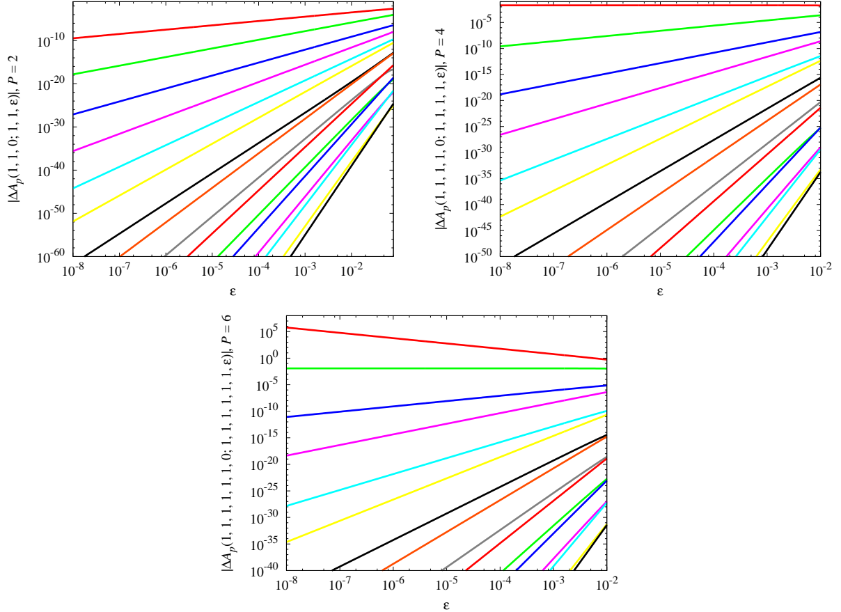
Figure 1: Deviations of diagonal transition amplitudes |\Delta A_p(\mathbf{a} = \mathbf{1}, t_a = 0; \mathbf{b} = \mathbf{1}, t_b = \varepsilon)| from the exact values as a function of propagation time \varepsilon for a multi-component system (36) of time-dependent harmonic oscillators: (top left) P = 2 oscillators, with \omega_1^2(t) = 1 + \frac{1}{2} \sin^2 2t , \omega_2^2(t) = 1 + \frac{1}{2} \cos 2t ; (top right) P = 4 oscillators, with \omega_1^2(t) , \omega_2^2(t) , \omega_3^2(t) = 2 + \cos 5t , \omega_4^2(t) = 4 + \sin^2 4t ; (bottom) P = 6 oscillators, with \omega_1^2(t) , \omega_2^2(t) , \omega_3^2(t) , \omega_4^2(t) , \omega_5^2(t) = 2 + \sin^2 t , \omega_6^2(t) = 4 + 2 \cos 3t . Each plot gives results for transition amplitudes calculated using the effective action levels p = 1, 2, \dots, 16 , from top to bottom.
