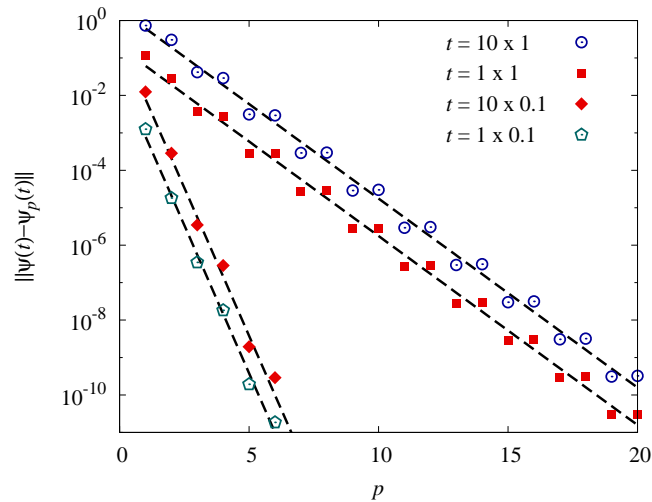
Figure 4: Integral measure (63) for numerically calculated time evolution of the harmonic oscillator as a function of the effective action level p for different values of the propagation time t . The parameters are the same as in Fig. 3.
