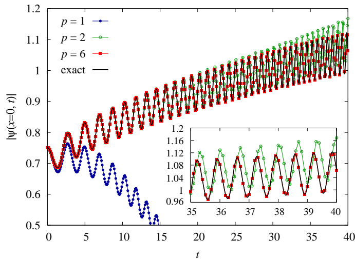
Figure 5: Time evolution of the time-dependent harmonic oscillator (64) calculated using the space-discretized method [46, 47] and the effective action approach with p = 1 , p = 2 , and p = 6 . The graph displays the time dependence |\psi(q = 0, t)| of the absolute value of the wave function at q = 0 . The time-dependent harmonic frequency is given by \omega(t) = 1 + \frac{1}{10} t , time-interval for propagation was \varepsilon = 0.1 , and the initial state was set according to Eq. (65).
