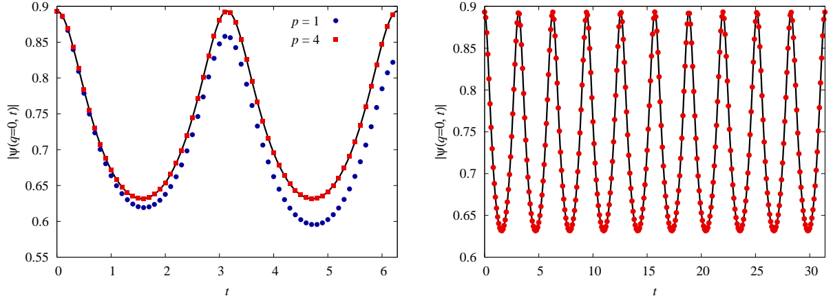
Figure 3: Time evolution of the one-dimensional harmonic oscillator V(q) = \frac{1}{2} \omega^2 q^2 calculated using the space-discretized method [46, 47] and the effective action approach with: (left) p = 1, 4 and (right) p = 20 . Both graphs display the time dependence |\psi(q = 0, t)| of the absolute value of the wave function at q = 0 , and solid line represents the exact solution. The harmonic frequency was \omega = 1 , the time-interval for propagation was \varepsilon = 0.1 , and the initial state was set to the ground state of the harmonic oscillator with \omega = 2 .
