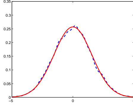
Figure 1: Comparison of the approximate density \hat{f}_h of \mathcal{E}_N (dotted line) with the density of \mathcal{N}(0, \sigma_F^2) , N = 5.10^5 , M = 5.10^3 , h = M^{-\frac{1}{5}} .
