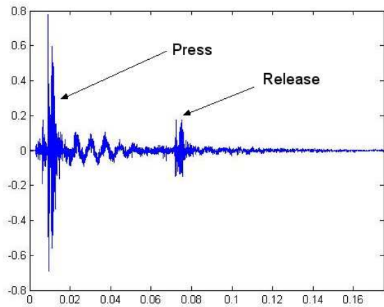
Fig. 1. Acoustic Signal of a Single Key
