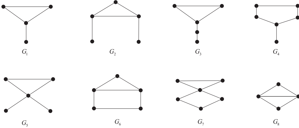
Figure 2: The graphs G_i , i=1, \dots, 8 .
