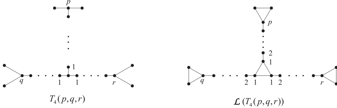
Figure 1: The graphs T_4(p, q, r) and \mathcal{L}(T_4(p, q, r)) where p, q, r \geq 1 .
