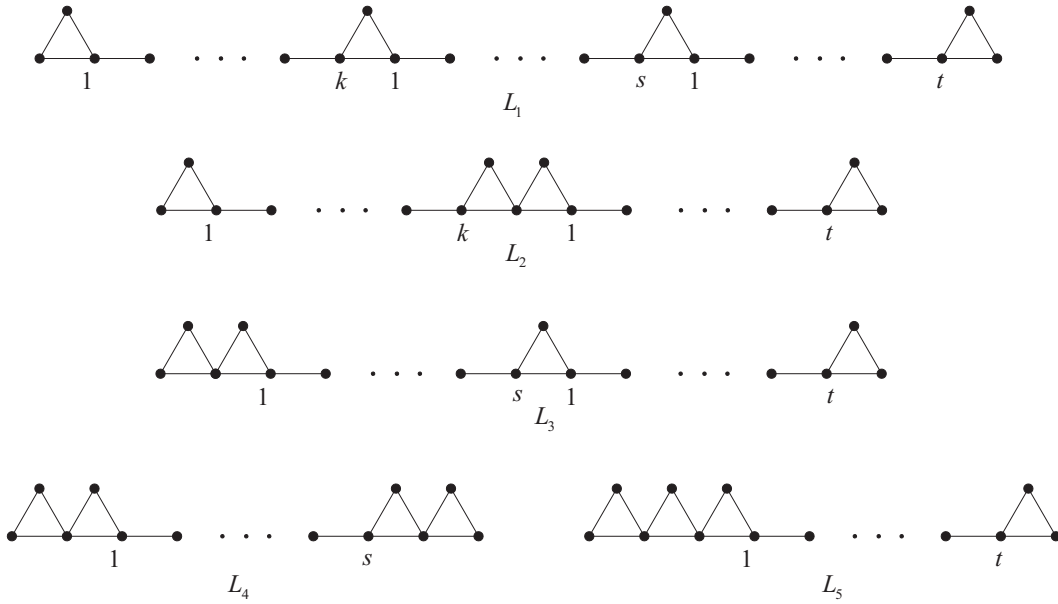
Figure 4: The graphs L_i , i = 1, \dots, 5 , where k, s, t > 1 .
