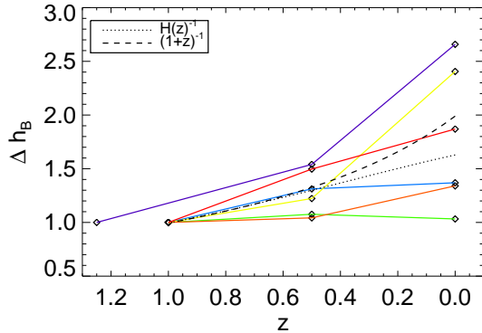
FIG. 8.— The growth of the simulated disks, normalized to their high z sizes. The dashed and dotted lines show simple predictions for the growth of disk galaxy populations since z=1 . The colors here are the same for individual galaxies as in Fig. 7.
