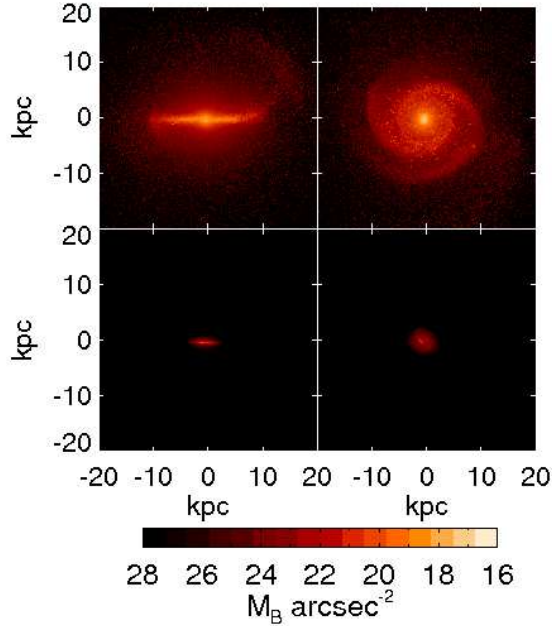
FIG. 1.— Galaxies h277 (top) and h799 (bottom), seen edge on (left) and face on (right) at z=0 in the B band. These galaxies span the full range of virial masses presented in this paper, two orders of magnitude.
