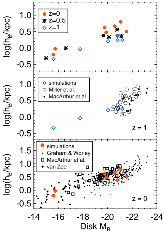
FIG. 5.— Rest frame B band disk scale length as a function of magnitude for our simulated galaxies. Top panel: The evolution of the population with time. Middle panel: Simulated points at z=1 as in the top panel, but now compared to observational results for decomposed disks from MacArthur et al. (2008) and Miller et al. ( in prep ). Bottom panel: Same as Fig. 4, shown again for comparison to the high z results.
