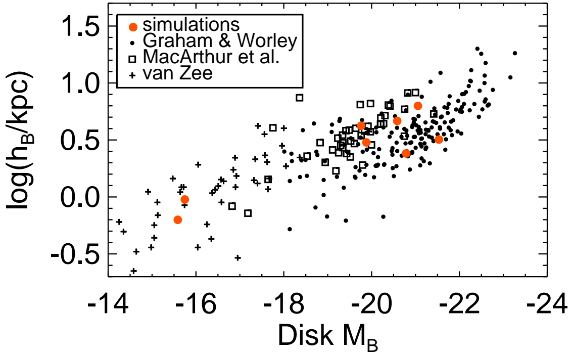
FIG. 4.— B band disk scale length as a function of magnitude for our simulated galaxies. Simulated galaxies at z=0 are shown as large red circles. The observational results of Graham & Worley (2008), MacArthur et al. (2003), and van Zee (2000) are shown for comparison.
