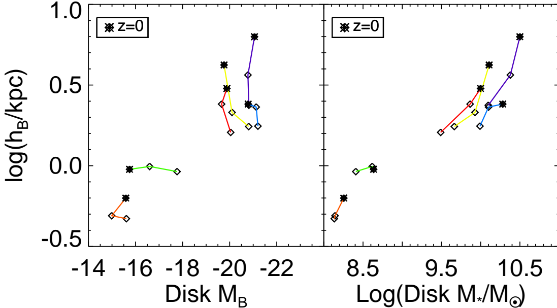
FIG. 7.— Left panel: Evolution in the magnitude – size plane with time. Each color connects an individual galaxy at z=1, 0.5 , and 0 . The higher z steps are marked by diamonds, and the z=0 step is indicated by a cross within the diamond. Note that low mass galaxies evolve more in luminosity (dimming), while higher mass galaxies evolve more in size. Right panel: Evolution in the stellar mass – size plane as a function of time. Note that these galaxies grow so that they remain on approximately the same relation with redshift.
