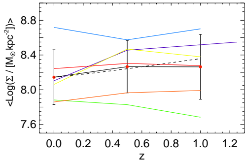
FIG. 9.— The surface mass density of the simulated disks as a function of redshift. The red points with error bars, connected by the solid black line, show the mean and standard deviation of the sample of nine at z = 0, 0.5 , and 1 . The mean varies by only 0.1 dex between z=1 and z=0 . The dashed line shows the analytic prediction for the SIS model. The colored lines show the evolution of each individual disk galaxy. Colors are the same for individual galaxies as in Figs. 7 and 8.
