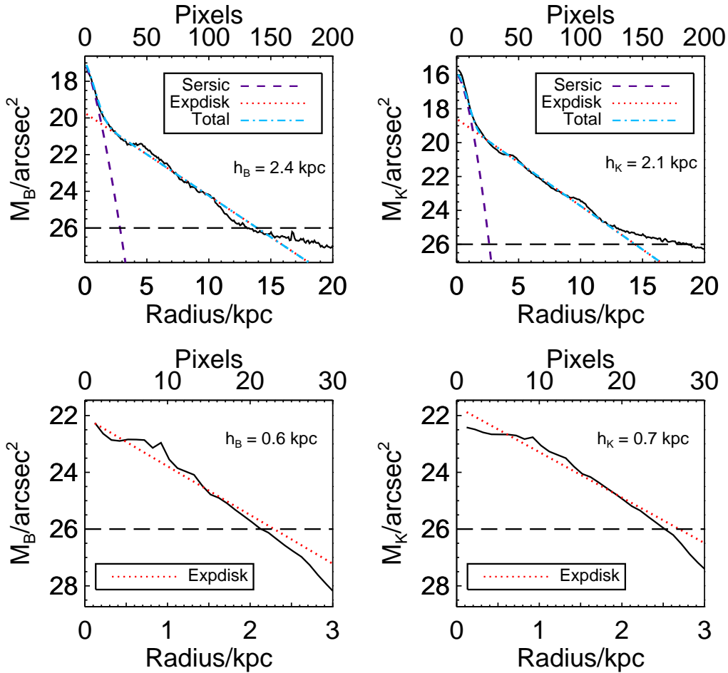
FIG. 2.— Face-on, radially averaged B band (left panels) and K band (right panels) surface brightness profiles (solid lines) at z=0 for the same galaxies as in Fig. 1 (h277 and h799). Bulge/disk decompositions resulting from GALFIT are shown, though the low mass galaxy in the bottom panel is bulgeless. The long dashed line in each panel at 26 M_B/\text{arcsec}^2 represents the limiting surface brightness out to which the profiles were fit.
