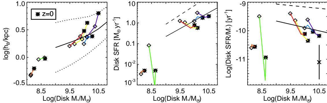
FIG. 11.— Comparison of simulated disk galaxy scaling relations to observational results. Left : The stellar mass – size relation, reproduced from the right panel of Fig. 7, now showing (solid line) the z=0 observed relation of Dutton et al. (2010b) plus the 2\sigma scatter in the observations (dotted lines). Their observed z=1 relation would simply be shifted downward 0.1 dex in size. Center : The stellar mass – SFR relation, as in Fig. 10, now showing the observed relations from Elbaz et al. (2007) at z=0 (solid line) and at z=1 (dashed line). Right : As for the center plot, but now for the sSFR. The x data point with error bars in the lower right corner of the panel represents roughly the 2\sigma scatter in the Elbaz et al. (2007) data.
