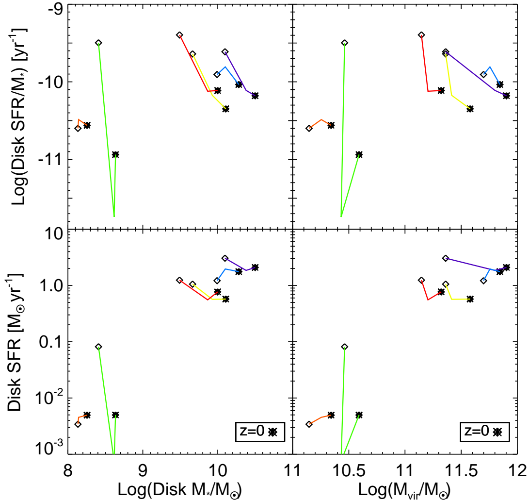
FIG. 10.— The SFR and sSFR of simulated galaxies. Left panels: The bottom panel shows the SFR in the disk of each galaxy as a function of the stellar disk mass. The top panel is the specific SFR of the disk. Right panels: Same as the left panels, but now in terms of the total virial mass of the halo. The colors here are the same for individual galaxies as in previous figures.
