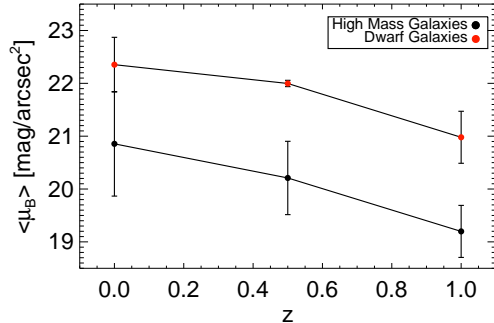
FIG. 6.— The evolution of surface brightness as a function of redshift. The two lowest mass galaxies are shown separately from the high mass galaxies. Data points at each z show the mean of the population, and the error bars reflect the standard deviation of the sample.
