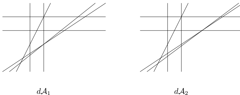
FIGURE 4. Arrangements that have homotopy equivalent complements. The fundamental group of the complement is not a direct sum of free groups.
