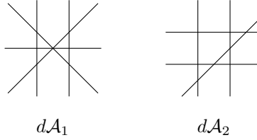
FIGURE 2. Arrangements from [Fal93] that have homotopy equivalent complements.
