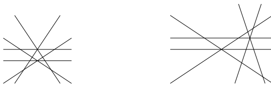
FIGURE 1. These arrangements have diffeomorphic complements and isomorphic lattices. The preferred arrangement is on the right.
