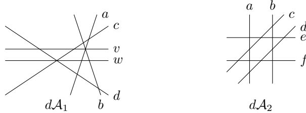
FIGURE 3. Arrangements that have homotopy equivalent complements.
