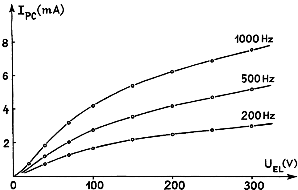
FIGURE 3 Dependence of the current I_{\text{PC}} on the voltage U_{\text{EL}} for U_{\text{PC}} 100 \text{ V}
