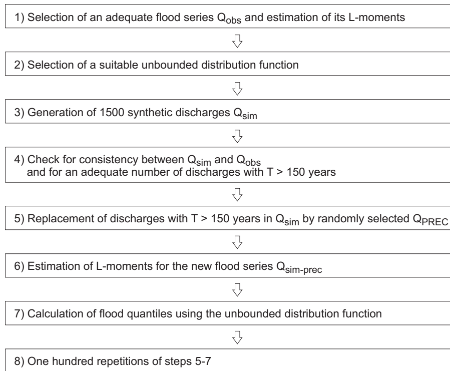
Fig. 5. Overview of the consecutive steps to integrate PREC flood quantiles into the at-site distribution function.
