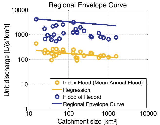
Fig. 3. Example of Regional Envelope Curve (REC) (from Guse et al., 2010).
