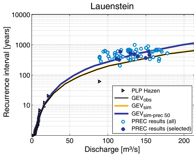
Fig. 6. Effect of integrating PREC flood quantiles into the at-site flood frequency analysis. GEV_{obs} , GEV_{sim} and GEV_{sim-prec} are compared for the site Lauenstein. The observed flood series is illustrated as Hazen plotting position (PLP Hazen). The PREC flood quantiles which were selected for GEV_{sim-prec} 50 are coloured in blue.
