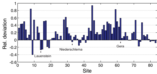
Fig. 8. Comparison of discharges estimated by GEV_{sim} and GEV_{sim-prec\ 50} for the target recurrence interval of 1000 years for 83 gauges. The three sites shown in Fig. 7 are marked.
