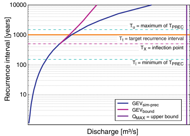
Fig. 4. Scheme of the proposed method including the most relevant variable names. The upper bound is illustrated in purple right of the legend. GEV_{sim-prec} is the combined distribution function of the observed flood series and the PREC flood quantiles. GEV_{bound} is a bounded distribution function which includes PREC flood quantiles as well as an upper bound discharge.
