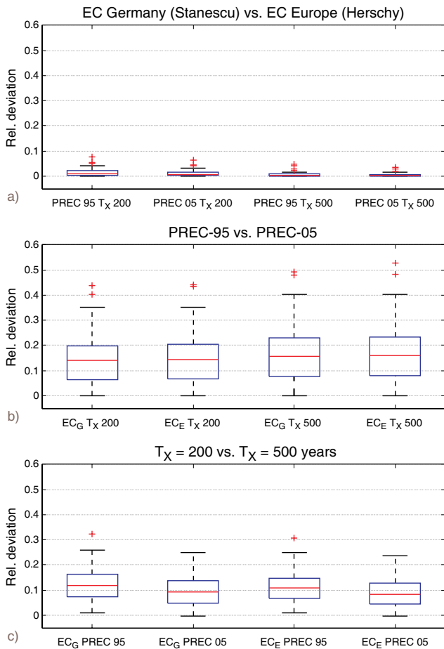
Fig. 10. Relative deviation between the quantile estimates of GEV_{bound} for T = 1000 years when varying three choices. The boxplots show the results for the 76 sites which were used in the sensitivity analysis. (a) Empirical envelope curves ( EC_G = Germany; Stanescu, 2002; EC_E = Europe; Herschy, 2002), (b) PREC flood discharges (95-, 5-quantiles) and (c) inflection point ( T_X ).
