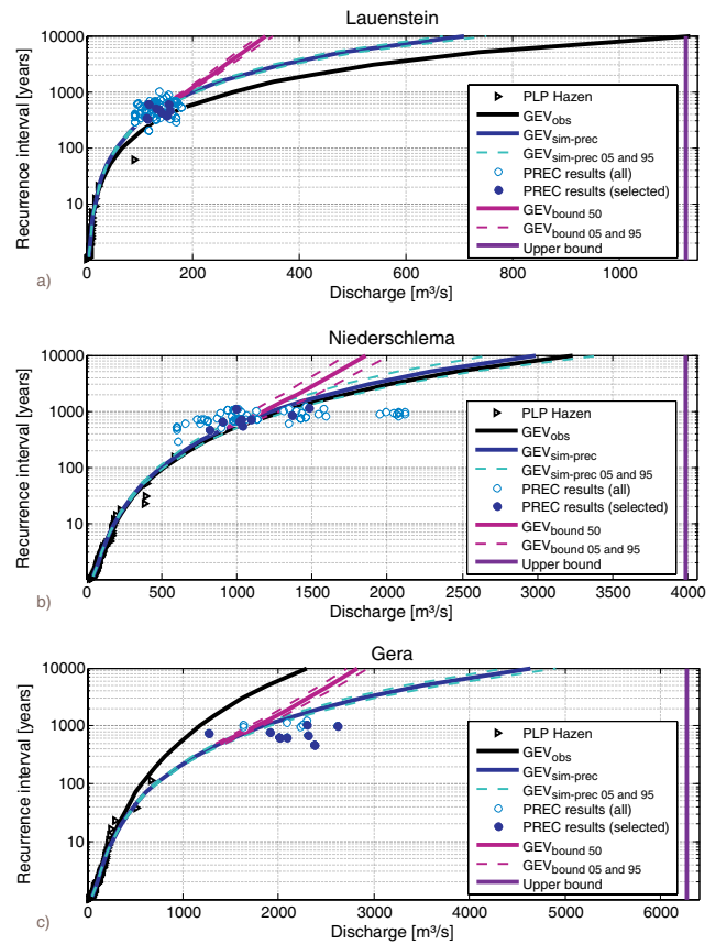
Fig. 7. The mixed bounded distribution function GEV_{bound} vs. the traditional GEV ( GEV_{obs} ) and the GEV_{sim-prec} for the gauges (a) Lauenstein, (b) Niederschlema, (c) Gera. The blue-coloured PREC results show the selected PREC discharges which yielded a median discharge for the target recurrence interval of 1000 years among the hundred repetitions. The upper bound is illustrated in purple right of the legend.
