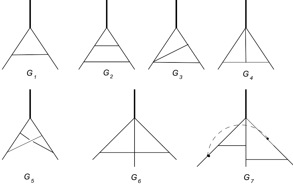
Figure 7: The set of scalar integrals. The arc line in G_7 corresponds to the presence of the numerator (k - p)^2 . Thick black line corresponds to off-shell leg with momentum q . All the other legs are on-shell.
