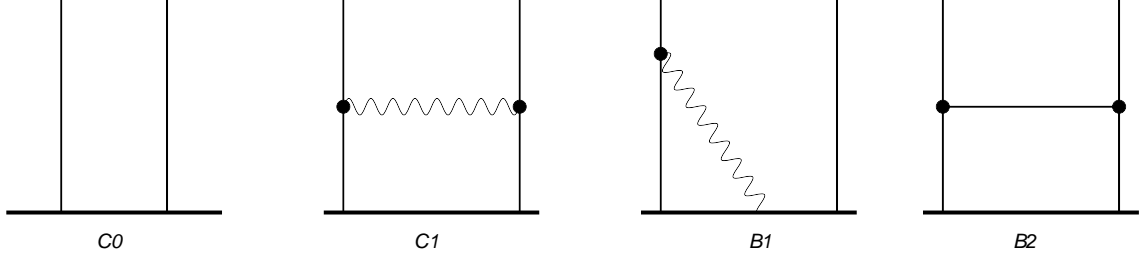
Figure 2: The relevant supergraphs. The internal black lines correspond to chiral propagators \langle \bar{\Phi}_I^a \Phi_J^b \rangle , wavy lines correspond to vector \langle V^a V^b \rangle propagator (see App. A). C0 is the tree level diagram, and the rest are one-loop ones. External lines are \Phi or \bar{\Phi} , and the lower bold line represents the insertion of the corresponding operator in modern notation. For the chiral operator \mathcal{C}_{IJ} only the diagrams C0 and C1 contribute, while for non-chiral operators \mathcal{V}_I^J and \mathcal{K} the other two ( B1 and B2 ) are also relevant.
