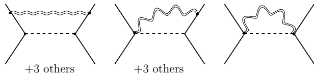
FIG. 5: Box diagrams.
