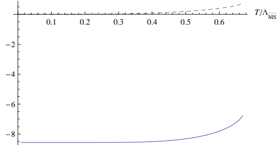
Fig. 1. The \langle g^2 A_\mu^2 \rangle condensate (full line) and the asymmetry \Delta_{A^2} (dashed line) as functions of the temperature, in units \Lambda_{\overline{\text{MS}}} .
