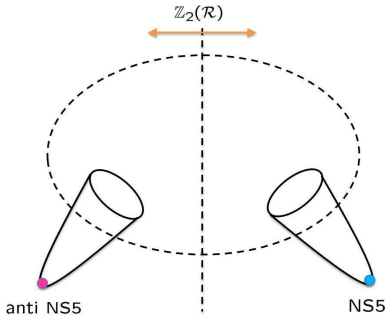
Figure 1: A schematic diagram of the internal space showing the two throats related by the \mathbb{Z}_2 \mathcal{R} symmetry containing the NS5-brane and the \overline{\text{NS5}} -brane respectively.
