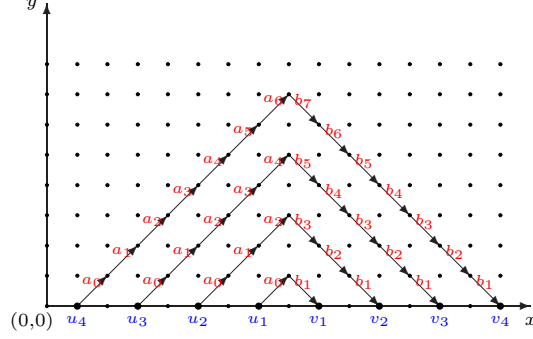
Figure 5: t = 1 and n = 4
