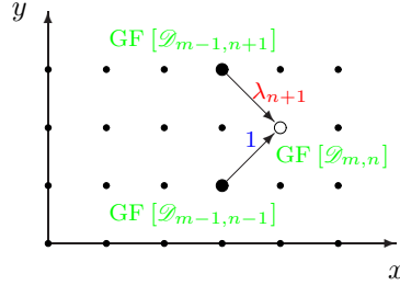
Figure 8: \text{GF}[\mathcal{M}_{m,n}] = \text{GF}[\mathcal{M}_{m-1,n-1}] + \lambda_{n+1}\text{GF}[\mathcal{M}_{m-1,n+1}]
