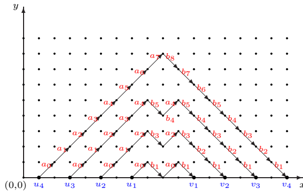
Figure 6: t = 1 and n = 4
