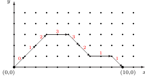
Figure 3: A Schröder path starting from (0,0) and ending at (10,0)
