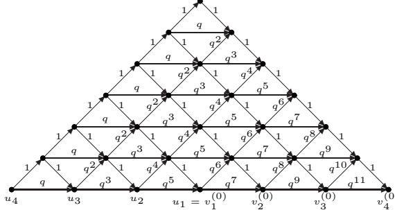
Figure 11: Weight of each edge
