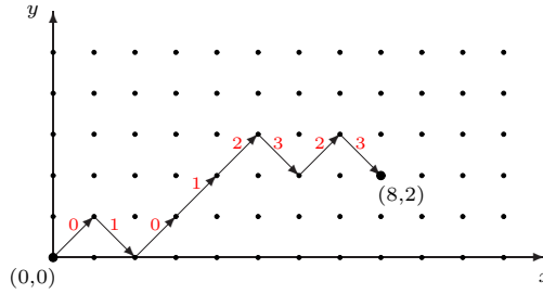
Figure 1: A Dyck Path starting from (0,0) and ending at (8,2)
