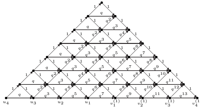
Figure 12: t = 1 case
