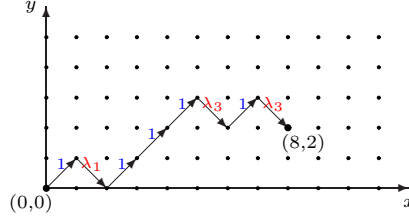
Figure 7: A Dyck Path of weight \lambda_1\lambda_3^2
