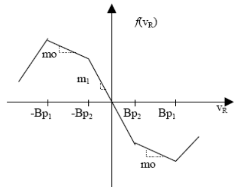
Fig. 2 Nonlinear term in Chua's circuit
