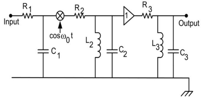
Fig. 3. Low-pass filter-mixer-two bandpass filters
