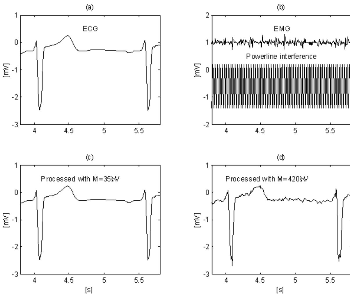
Figure 13 Interference+EMG noise suppression using adaptive threshold M: 'clean signal' (a) processed with M = 35 \mu V (c) and contaminated signal (b) subjected to the procedure with M = 420 \mu V (d).
