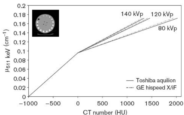
Figure 13. Calculated bi-linear calibration curves for conversion of CT numbers (HU) into linear attenuation coefficients at 511 keV at different tube voltages for both Aquilion and HiSpeed X/iF CT scanners. Reprint with permission from ref. [57].
