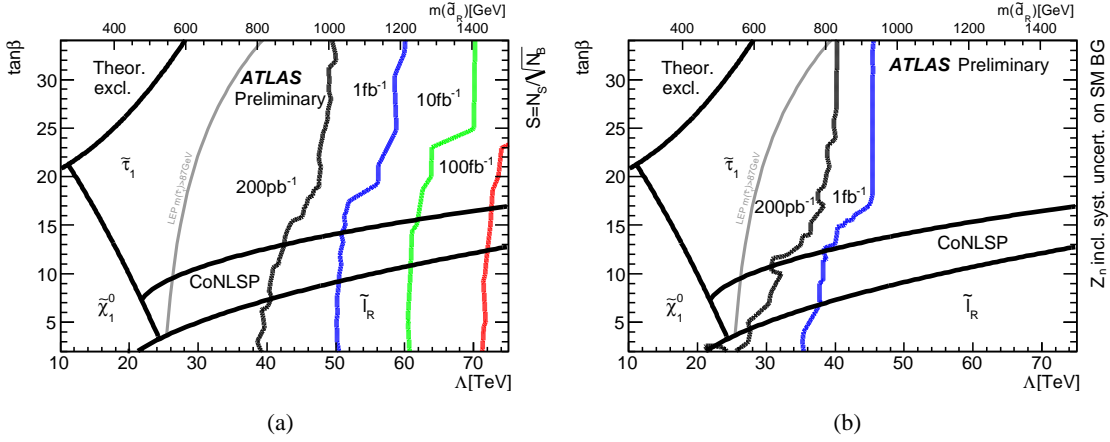
Figure 1: Integrated luminosity needed for a signal significance of S = 5 or Z_n = 5 , respectively, in the (\Lambda\text{-tan}\beta) -plane for M_m = 250\text{ TeV} , N_5 = 3 , \text{sgn}\mu = + and C_{\text{grav}} = 1 using (a) the simple calculation of the significance S and (b) Z_n properly including the systematic uncertainties.
