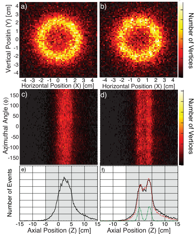
Figure 3: (a-b) Azimuthal projections of the \bar{p} annihilation vertex distributions during mixing with (a) no neutral atom trap and (b) the full trap. (c-d) Corresponding z - \phi distributions. (e-f) Corresponding axial ( z ) distributions. (f) Dashed (red): Fit to the distribution, see text; Dot-dashed (green) peaks in fit. The shaded area marks the three layer part of the detector used for tracking. Left of this area the detector has only one layer of silicon. The slight asymmetry in the axial distributions (in particular the tails) is due to the lower reconstruction efficiency outside the three layer section. For clarity the plots have been normalized to have the same total number of events. The zero axial position is the center of the neutral atom trap.
