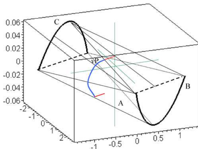
Figure A.1. The Elfving set defined in (A.2) for the parameters a = 0.133 , b = 0.272 , \gamma = 3.33 . The points f(d_1) , -f(d_2) and f(d_3) are denoted by A , C and B , respectively, while the point \nu P is defined in (A.1).
