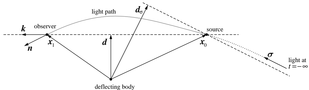
Figure 1. Definitions of vectors \mathbf{x}_1 , \mathbf{x}_0 , \mathbf{k} , \mathbf{n} , \boldsymbol{\sigma} . Vectors \mathbf{d} (defined in Section 4.1) and \mathbf{d}_\sigma (defined in Section 5.4) are also shown.
