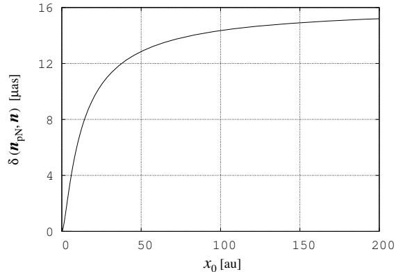
Figure 2. The angle between \mathbf{n}_{\text{pN}} and \mathbf{n} for Jupiter. The vector \mathbf{n}_{\text{pN}} is evaluated by means of the standard post-Newtonian formula (24), while \mathbf{n} is taken from the numerical integration as described in Section 3. Impact parameter d is taken to be the radius of Jupiter and the distance x_1 between Jupiter and the observer is 6 au.
