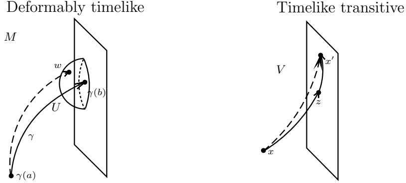
Figure 5: Examples of deformably timelike curve (left) and timelike transitive point (right).
