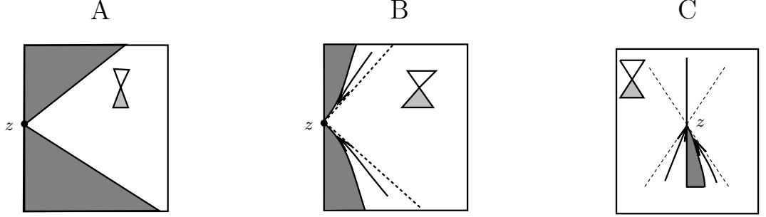
Figure 6: In Figure (A), point z is not accessible, because it is not reachable by a timelike curve from M . In Figure (B), any timelike curve reaching z must be null at z , i.e. z is future and past accessible, but not strongly accessible. In Figure (C), point z is the endpoint of two future-directed timelike curves, one of them is strongly timelike and the other one is not.
