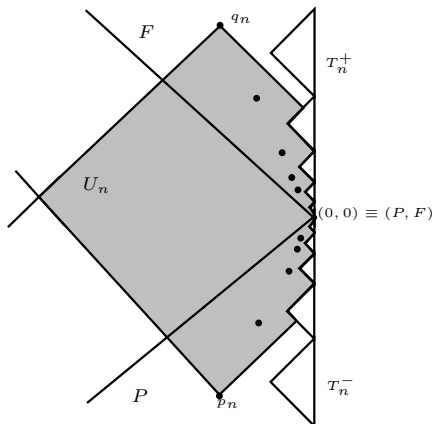
Figure 2: The origin corresponds with a pair (P, F) \in \partial M which does not have a sequentially compact neighborhood (see Example 3.30). Any open neighborhood U_n = I^+(p_n, \bar{M}) \cap I^-(q_n, \bar{M}) \subset \bar{M} of (P, F) contains a sequence with no limit in \bar{M} .
