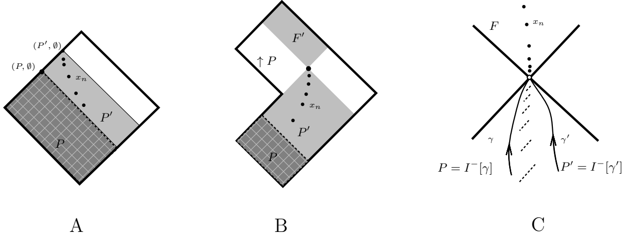
Figure 1: In Figure (A) the sequence \{x_n\}_n converges to both (P, \emptyset) , (P', \emptyset) with CEAT, but does not converge to (P, \emptyset) with any topology satisfying (A1), (A2) in Defn. 3.18 (requirement (A3) ensures the convergence to (P', \emptyset) ). Analogously, in Figure (B) the sequence \{x_n\}_n converges to both (P, \emptyset) , (P', F') with CEAT, but does not converge to (P, \emptyset) if (A1), (A2) are fulfilled. In Figure (C), the sequence \{x_n\}_n (as well as the sequence constantly equal to (P', F) ) converges to both (P', F) , (P, \emptyset) with the Marolf-Ross topology, but only converges to (P', F) with the chronological topology.
