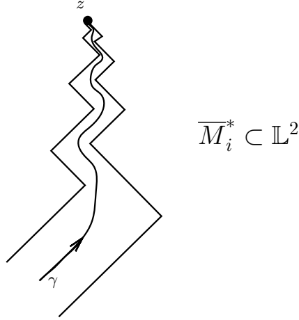
Figure 4: Because of the infinity breaks of \partial_i^* M , the causal curve \gamma , which is smooth in M , cannot be smoothly extended to z \in \partial_i^* M . The extended curve is causal continuous because there are close smooth causal curves in M_0 which connect any point of \gamma with z . Nevertheless, no such curves are contained in \overline{M}_i^* . Any point p on \gamma satisfies p \ll_i^W z , but p \not\ll_i^S z .
