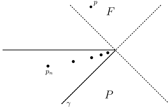
Figure 3: Non-properly causal completion for any admissible boundary.
