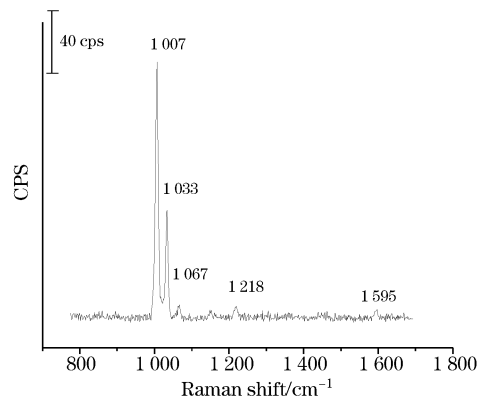
Fig. 3 SERS of pyridine ( 0.01 \text{ mol} \cdot \text{L}^{-1} ) from silver nanocubes assembled on silicon wafer. The edge length of silver nanocubes is 320-330 nm. Excitation line: 632.8 nm
