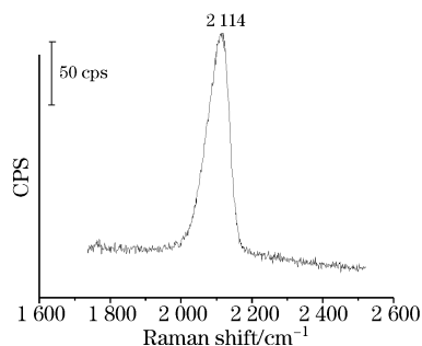
Fig. 4 SERS of \text{SCN}^- ( 0.01 \text{ mol} \cdot \text{L}^{-1} ) from silver nanocubes assembled on silicon wafer. The edge length of silver nanocubes is 320-330 nm. Excitation line: 632.8 nm
