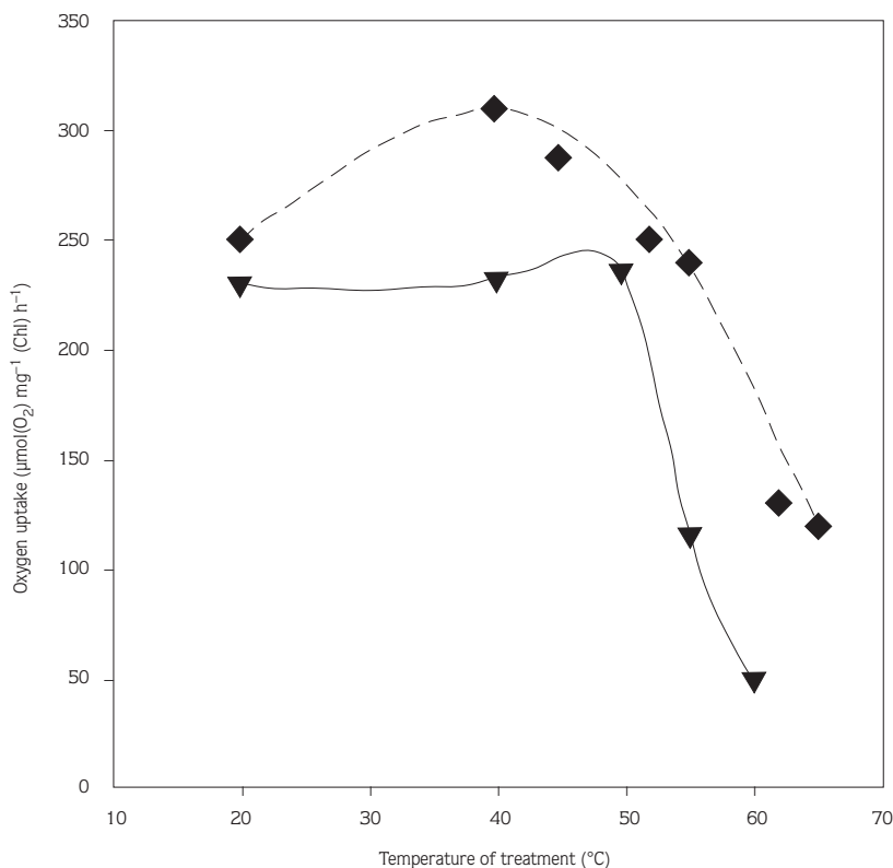
Figure 4. Dependence on incubation temperature of the rate of electron transport from DQH 2 to MV in thylakoid membranes. Thylakoid membranes were incubated for 10 min at designated temperatures in 25 mM HEPES-NaOH (pH 7.5), 10 mM NaCl, 0.4 M sucrose and then cooled to 20°C. After the addition of 0.01 mM DCMU, 0.5 mM DQH 2 , 0.2 mM MV, 75 units/ml SOD the electron-transport activity was measured by monitoring of oxygen uptake. ▼—no betaine added to both the preparation and incubation mixtures. ◆—0.5 M betaine was added to these mixtures. Each point represents the mean of 3 experiments.
