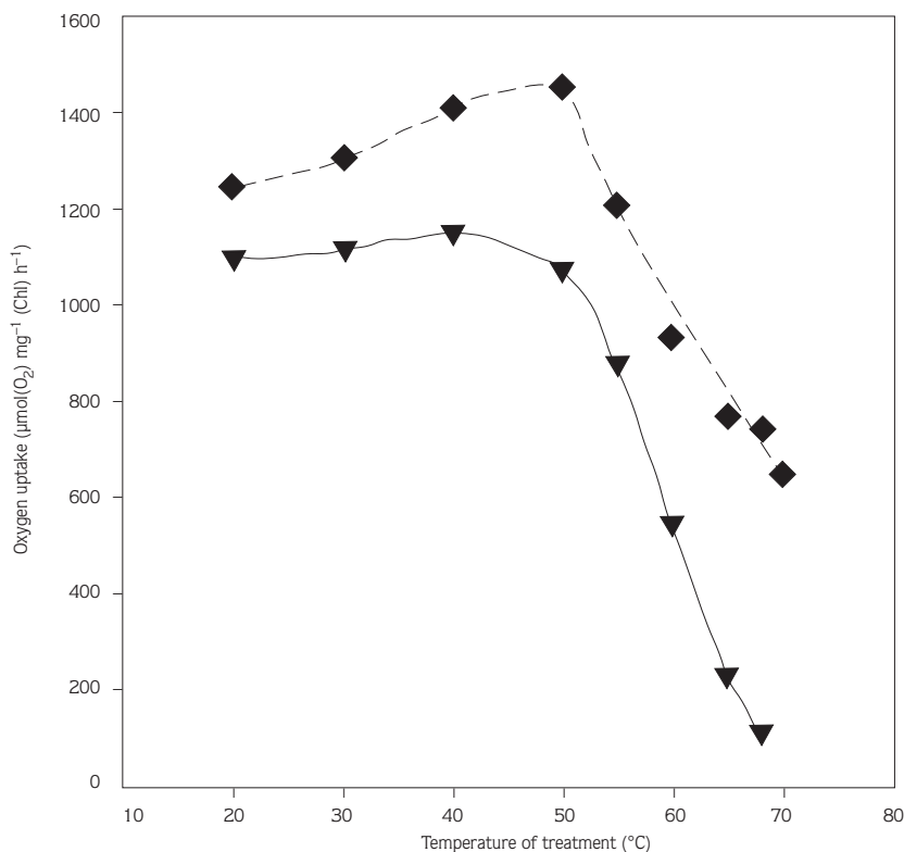
Figure 5. Dependence on incubation temperature of the rate of electron transport from DAD to MV in thylakoid membranes. Thylakoid membranes were incubated for 10 min at designated temperatures in 25 mM HEPES-NaOH (pH 7.5), 10 mM NaCl, 0.4 M sucrose and then cooled to 20°C. After the addition of 0.01 mM DCMU, 0.5 mM DAD, 1 mM Na-ascorbate, 0.2 mM MV, 75 units/ml SOD the electron-transport activity was measured by monitoring of oxygen uptake. ▼—no betaine added to both the preparation and incubation mixtures. ◆—0.5 M betaine was added to these mixtures. Each point represents the mean of 3 experiments.
