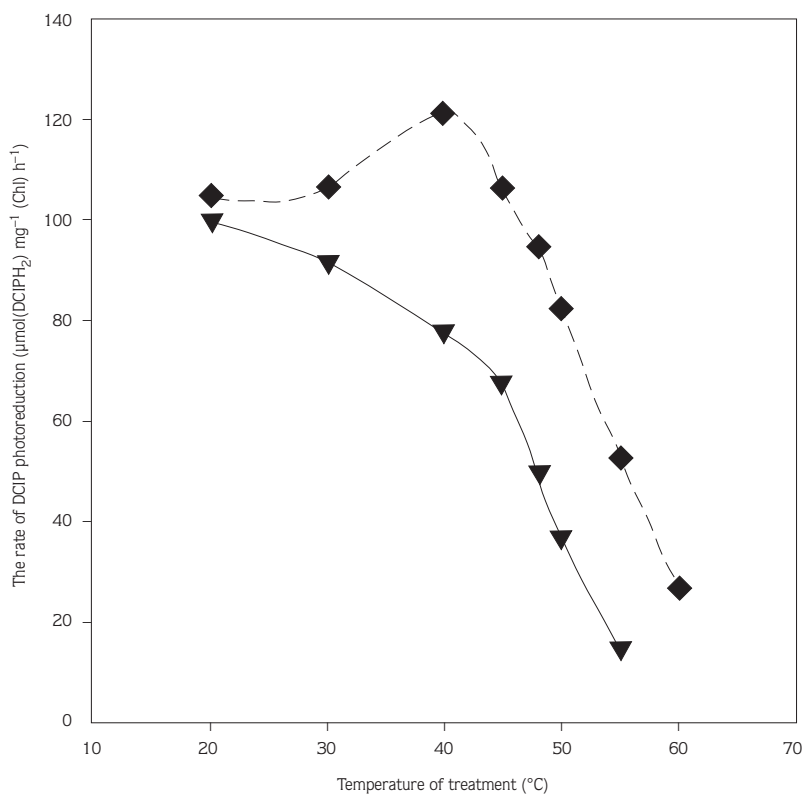
Figure 3. Dependence on incubation temperature of the rate of electron transport from H_2O + DPC to DCIP in thylakoid membranes. Thylakoid membranes were incubated for 10 min at designated temperatures in 25 mM HEPES-NaOH (pH 7), 10 mM NaCl, 0.4 M sucrose and then cooled to 20°C. After the addition of 0.05 mM HClP, 0.5 mM DPC the electron-transport activity was measured by monitoring the photoreduction of DCIP. ▼—no betaine added to both the preparation and incubation mixtures. ◆—0.5 M betaine was added to these mixtures. Each point represents the mean of 3 experiments.
