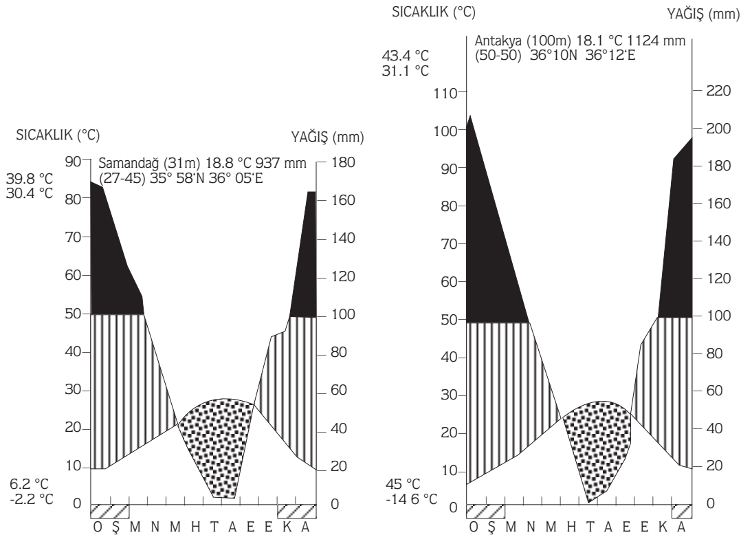
Figure 2. Climatic diagrams of Samandağ and Antakya.
