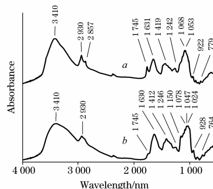
Fig. 1 FTIR spectra of radix isatidis
