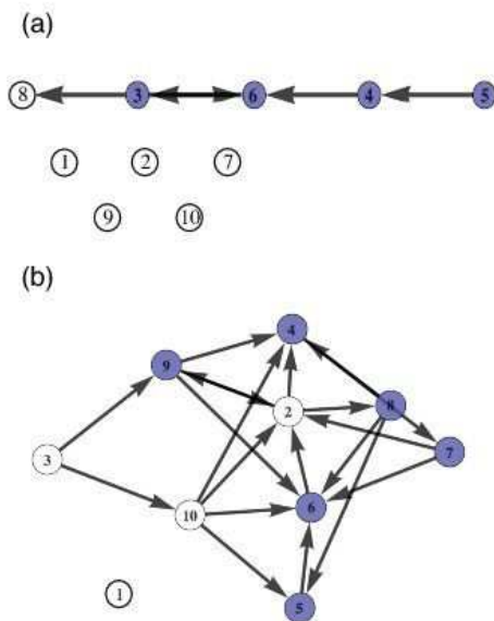
FIG. 4: (Color online). Two typical realizations of the synchronization-optimized network at different connectivities (a) p = 0.05 and (b) p = 0.2 . The blue (gray) nodes indicate entrained oscillators. The numbers in the nodes are indexes of the oscillators. The parameters are N = 10 , \beta = \beta_M , M = 11 , and \delta\beta = 10 .
