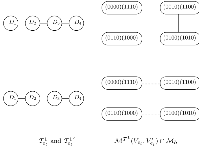
Figure 8. The structure of \mathcal{M}_{\mathbf{b}}^{T^1} .
