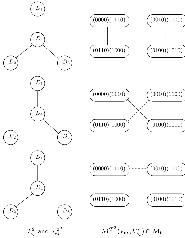
Figure 9. The structure of \mathcal{M}_b^{T^2} .
