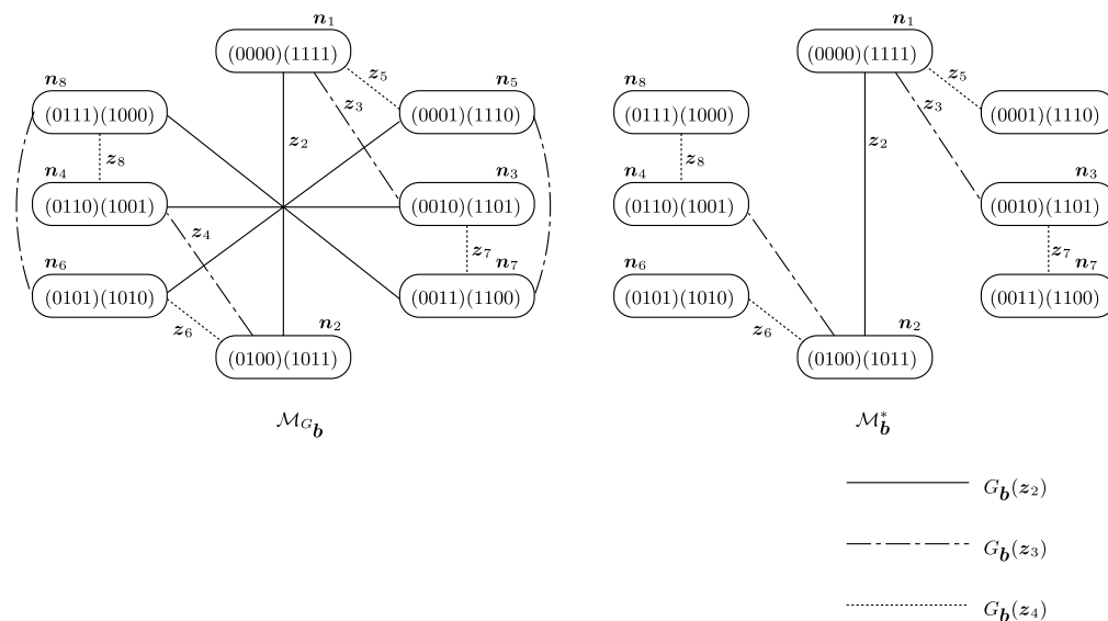
Figure 11. \mathcal{M}_{G_{\mathbf{b}}} and \mathcal{M}_{\mathbf{b}}^* generated by Algorithm 1.
