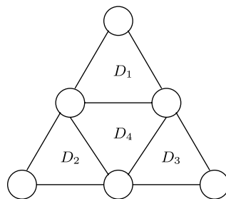
Figure 10. A chordal graph whose clique tree is uniquely determined.
