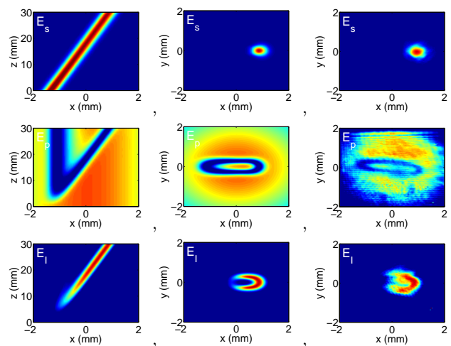
FIG. 6: Solitary regime. Left column, numerical dynamics of the beams E_s , E_p , E_i in the x - z ( y = 0 ) plane. Central column, numerical, and right column, experimental results at the exit face of the KTP crystal presenting the spatial x - y output profiles of the beams. At the input I_s = 50MW/cm^2 , I_p = 0.1MW/cm^2 .
