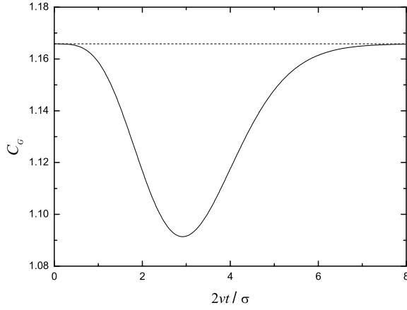
Figure 1: Statistical complexity, C_G , vs. the adimensional separation, 2vt/\sigma , between the two traveling Gaussian densities defined in Eq. (6). The minimum of C_G is reached when 2vt/\sigma = 2.91 . The dashed line indicates the value of complexity for the normalized Gaussian distribution.
