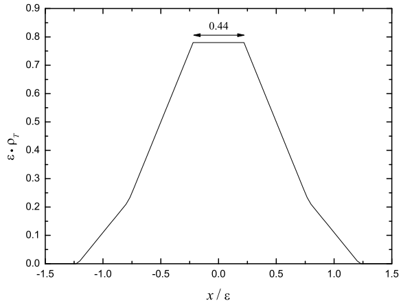
Figure 6: Shape of the density (1) in adimensional units that presents the maximum statistical complexity when the two traveling triangular densities defined in (9) are crossing. Notice that the value of the adimensional separation between the centers of both triangular distributions must be 0.44.
