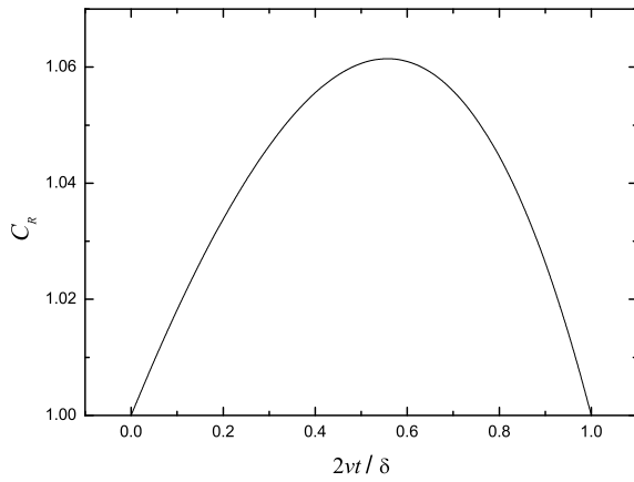
Figure 3: Statistical complexity, C_R , vs. the adimensional separation, 2vt/\delta , between the two traveling rectangular densities defined in Eq. (7). The maximum of C_R is reached when 2vt/\delta = 0.557 . Observe that the normalized rectangular distribution has C_R = 1 .
