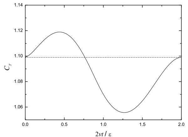
Figure 5: Statistical complexity, C_T , vs. the adimensional separation, 2vt/\epsilon , between the two traveling triangular densities given in Eq. (9). The maximum and minimum of C_T are reached when 2vt/\epsilon takes the values 0.44 and 1.27, respectively. The dashed line indicates the value of complexity for the normalized triangular distribution.
