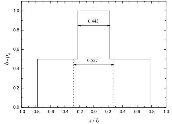
Figure 4: Shape of the density (1) in adimensional units that presents the maximum statistical complexity when the two traveling rectangular densities defined in (7) are crossing. Notice that the value of the adimensional separation between the centers of both rectangular distributions must be 0.557. Then, the width of the overlapping between both distributions is 0.443.
