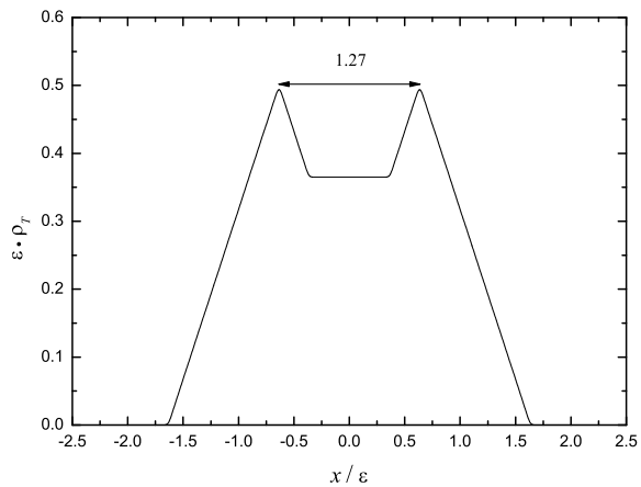
Figure 7: Shape of the density (1) in adimensional units that presents the minimum statistical complexity when the two traveling triangular densities defined in (9) are crossing. Notice that the value of the adimensional separation between the centers of both triangular distributions must be 1.27.
