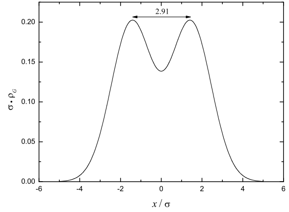
Figure 2: Shape of the density (1) in adimensional units that presents the minimum statistical complexity when the two traveling Gaussian densities defined in (6) are crossing. Notice that the value of the adimensional separation between the centers of both Gaussian distributions must be 2.91.
