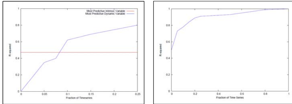
Fig. 4. Sample music market prediction results. The plot at left shows the fraction of final market share variance explained by the most predictive intrinsic alone ( \alpha ms_{i, noSI} , red) and most predictive dynamics variable alone ( \beta_2 ms_i(k\tau) , blue), as a function of the fraction of early time series available. The plot at right depicts the fraction of final market share variance explained by \Sigma_{ms} as a function of the fraction of early time series available.
