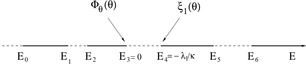
Figure 2: The spectrum of the operator -\hat{Q}_{[X,T]}/k . The intervals [E_0, E_1] , [E_2, E_3] , [E_4, E_5] and [E_1, E_2] , [E_3, E_4] , [E_5, E_6] represent the energy bands and the energy gaps of a finite size respectively.
