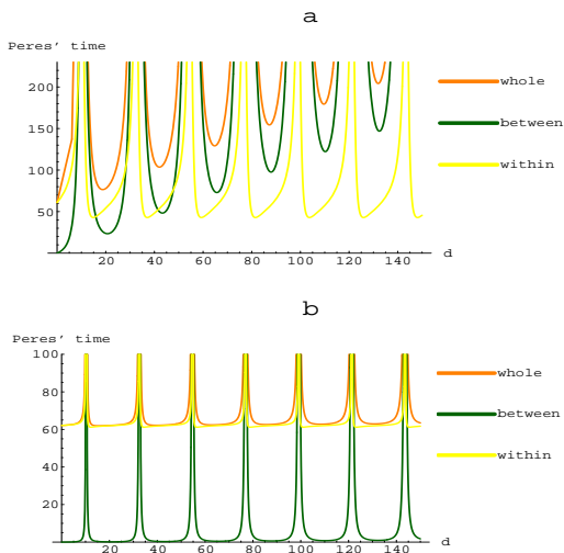
FIG. 1: (Color online) Peres' clock time dependence with respect to the distance d between the two barriers. In both figures the three clock times appearing in relation (16) are shown, corresponding to the whole potential region (0, 2a+d) , to the region between the barriers (a, a+d) , and to the region within the two barriers (0, a) \cup (a+d, 2a+d) . Natural units were used ( \hbar = c = 1 ), so that mass and energies are expressed in units of the particle mass \mu , and distances and times are expressed in units of \mu^{-1} . In both figures E = 0.01 and V_0 = 0.018 . (a) a = 10 ; (b) a = 30 .
