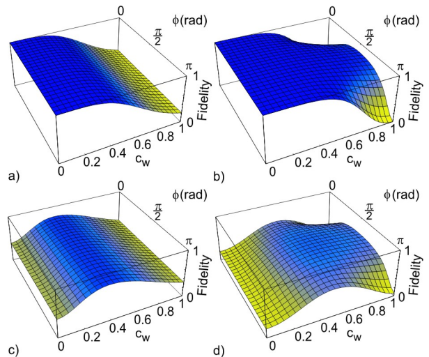
FIG. 5: (Color online) Calculated fidelity of W_4 (a) and GHZ_4^+ (b) states when considering only five photon contributions (Eq. 9). Calculated fidelity of W_4 (c) and GHZ_4^+ (d) states when considering also six photon contributions. All calculations assume a strength of the SPDC source of |z_{dc}| = 0.17 , which we experimentally observed for our setup.
