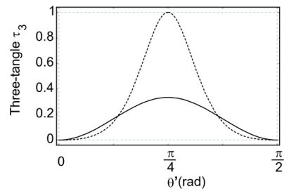
FIG. 1: Three-tangle \tau_3 for the states of Eq. 1 without (straight) and with (dashed) application of the transformation \mathcal{T}_+ \otimes \mathcal{T}_+ \otimes \mathcal{T}_+ (where \alpha' = \cos \theta' and \epsilon' = 0 ).
