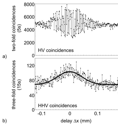
FIG. 4: Coherence between the weak coherent beam and the SPDC photons. (a) Interference of the two possibilities how to obtain an HV coincidence. (b) Enhanced emission (cloning) due to bosonic nature of photons. The solid line shows a Gaussian fit to the data points giving an enhancement of 1.52 \pm 0.03 .
