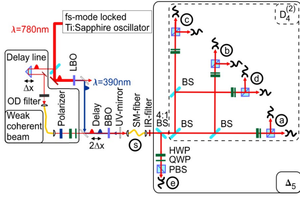
FIG. 2: (Color online) Schematic experimental set-up for the observation of the state |D_4^{(2)}\rangle (innermost section, dashed frame). The weak coherent beam, the 4:1 beam splitter as well as the detection in an additional mode e are needed for the proposed experimental implementation of the five photon states |\Delta_5\rangle (details see text).
