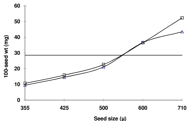
Figure 1. Relationships between sieve graded seed size and 100-seed weight of two tef varieties ( \Delta DZ-01-974; \square DZ-Cr-37) and mean of the ungraded controls (-).
